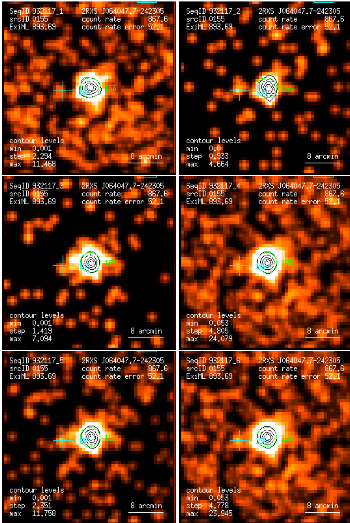
Figure 155: RASS 932117: detection 0155: band rate images, Gaussian filter: (1) PSPC channels 11 – 41, (2) 52 – 90, (3) 91 – 201, (4) 11 – 235, (5) 52 – 201, (6) 11 – 201. Broad band rates in counts/ks. Band rate contour levels in counts/ks/arcmin 2 .
