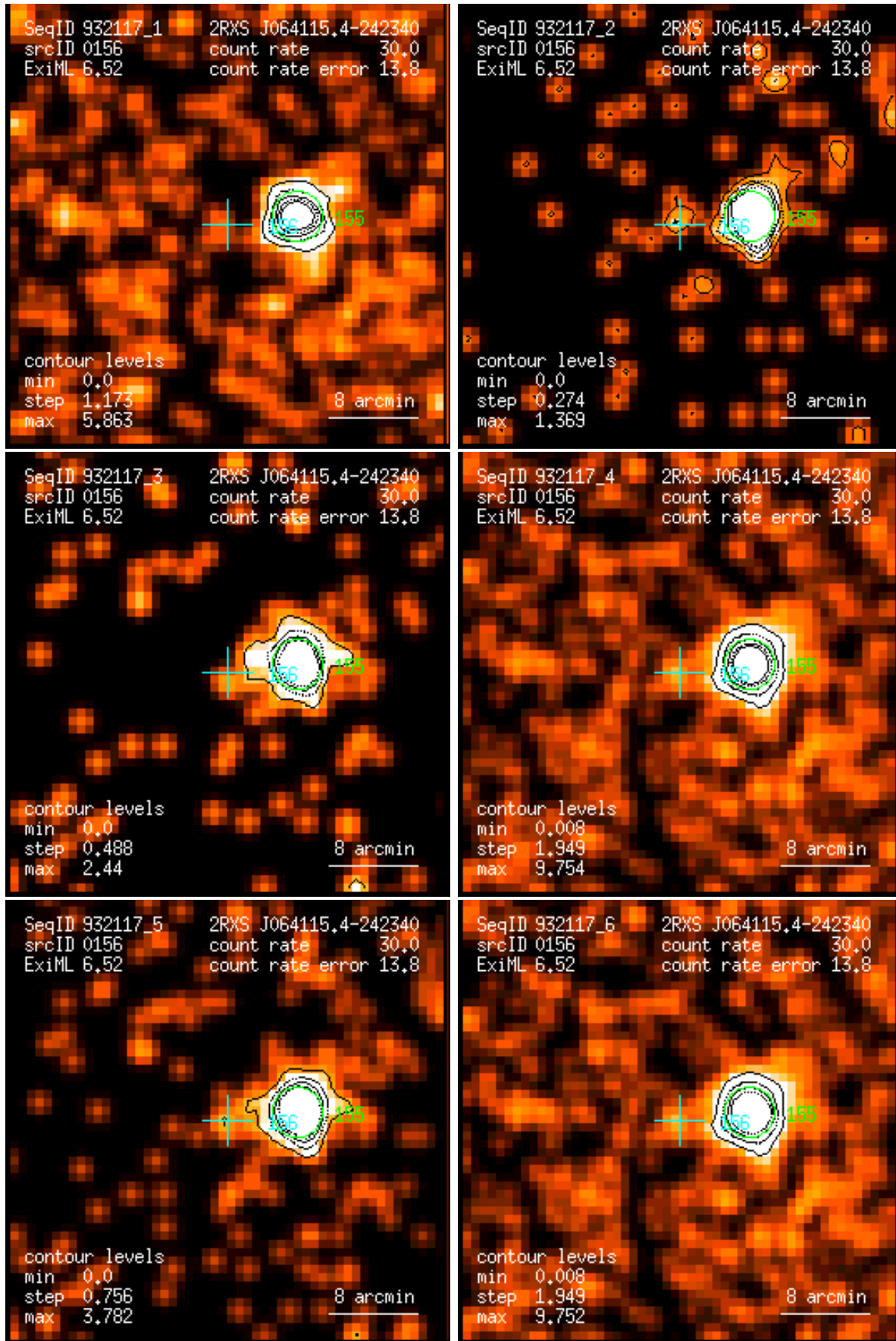
Figure 156: RASS 932117: detection 0156: band rate images, Gaussian filter: (1) PSPC channels 11 – 41, (2) 52 – 90, (3) 91 – 201, (4) 11 – 235, (5) 52 – 201, (6) 11 – 201. Broad band rates in counts/ks. Band rate contour levels in counts/ks/arcmin 2 .
