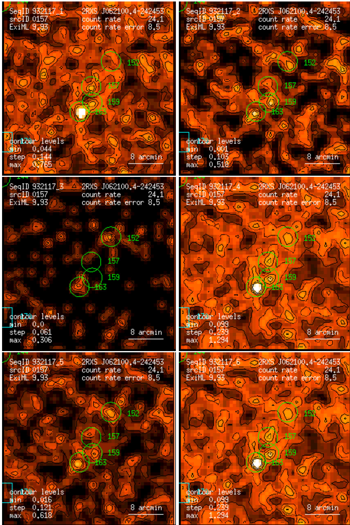
Figure 157: RASS 932117: detection 0157: band rate images, Gaussian filter: (1) PSPC channels 11 – 41, (2) 52 – 90, (3) 91 – 201, (4) 11 – 235, (5) 52 – 201, (6) 11 – 201. Broad band rates in counts/ks. Band rate contour levels in counts/ks/arcmin 2 .
