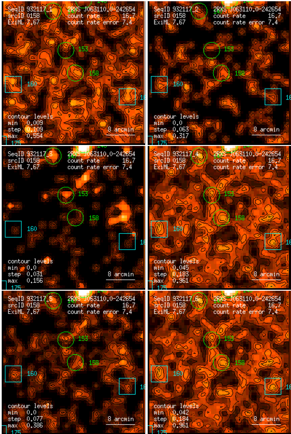
Figure 158: RASS 932117: detection 0158: band rate images, Gaussian filter: (1) PSPC channels 11 – 41, (2) 52 – 90, (3) 91 – 201, (4) 11 – 235, (5) 52 – 201, (6) 11 – 201. Broad band rates in counts/ks. Band rate contour levels in counts/ks/arcmin 2 .
