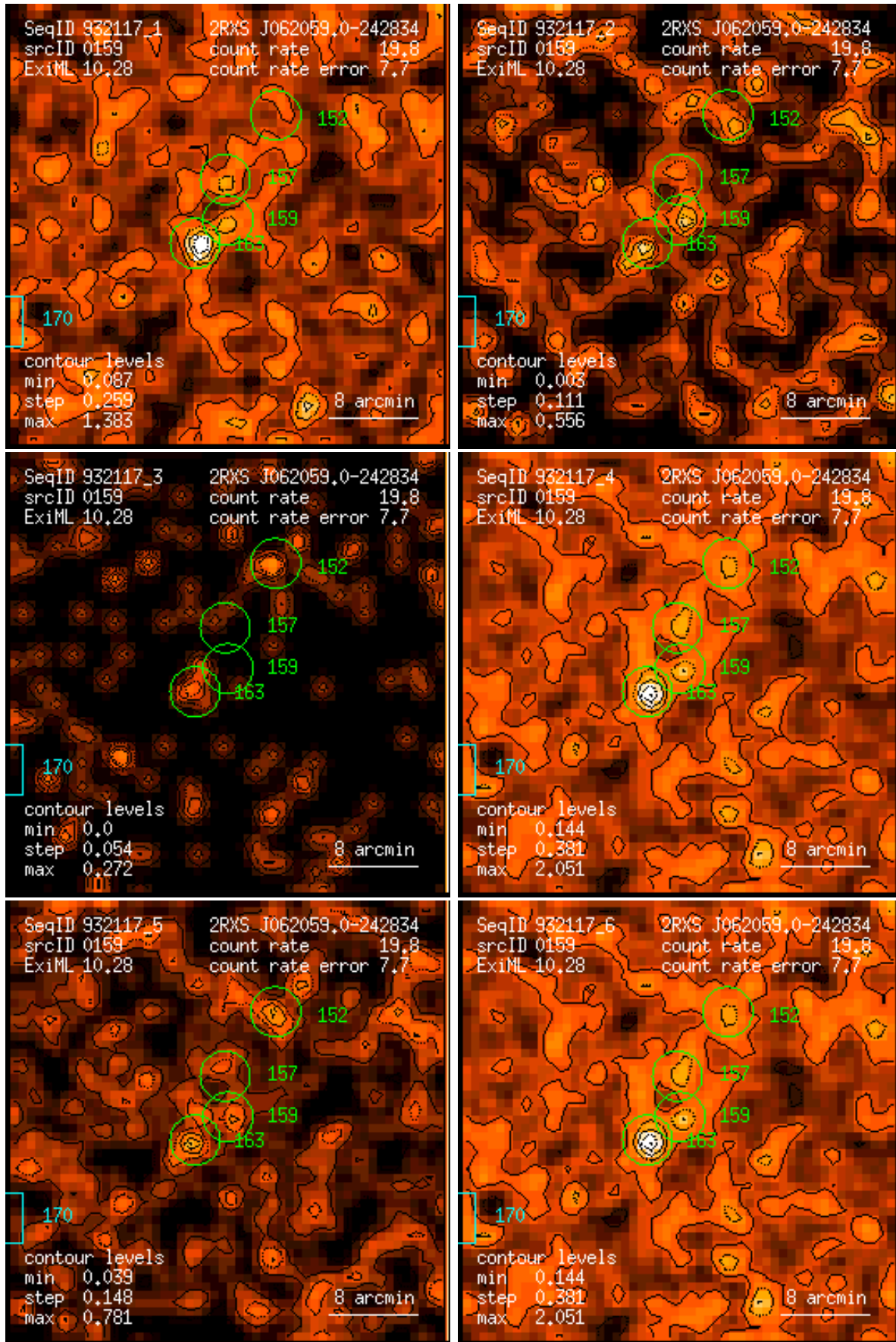
Figure 159: RASS 932117: detection 0159: band rate images, Gaussian filter: (1) PSPC channels 11 – 41, (2) 52 – 90, (3) 91 – 201, (4) 11 – 235, (5) 52 – 201, (6) 11 – 201. Broad band rates in counts/ks. Band rate contour levels in counts/ks/arcmin 2 .
