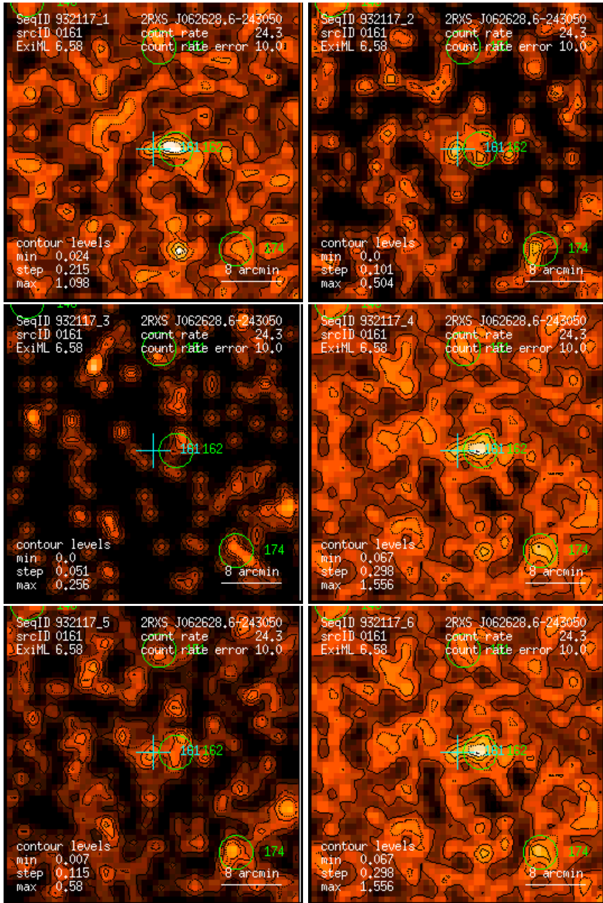
Figure 161: RASS 932117: detection 0161: band rate images, Gaussian filter: (1) PSPC channels 11 – 41, (2) 52 – 90, (3) 91 – 201, (4) 11 – 235, (5) 52 – 201, (6) 11 – 201. Broad band rates in counts/ks. Band rate contour levels in counts/ks/arcmin 2 .
