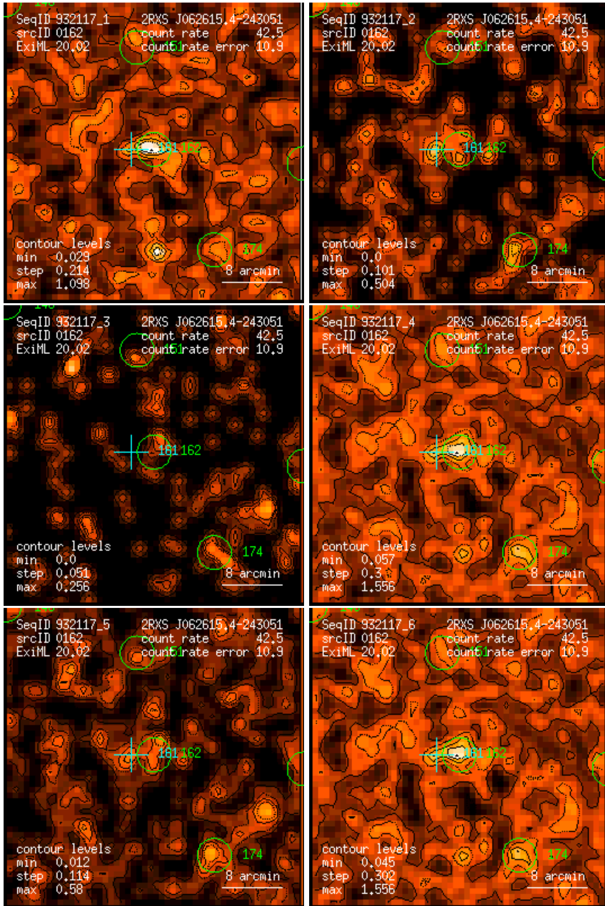
Figure 162: RASS 932117: detection 0162: band rate images, Gaussian filter: (1) PSPC channels 11 – 41, (2) 52 – 90, (3) 91 – 201, (4) 11 – 235, (5) 52 – 201, (6) 11 – 201. Broad band rates in counts/ks. Band rate contour levels in counts/ks/arcmin 2 .
