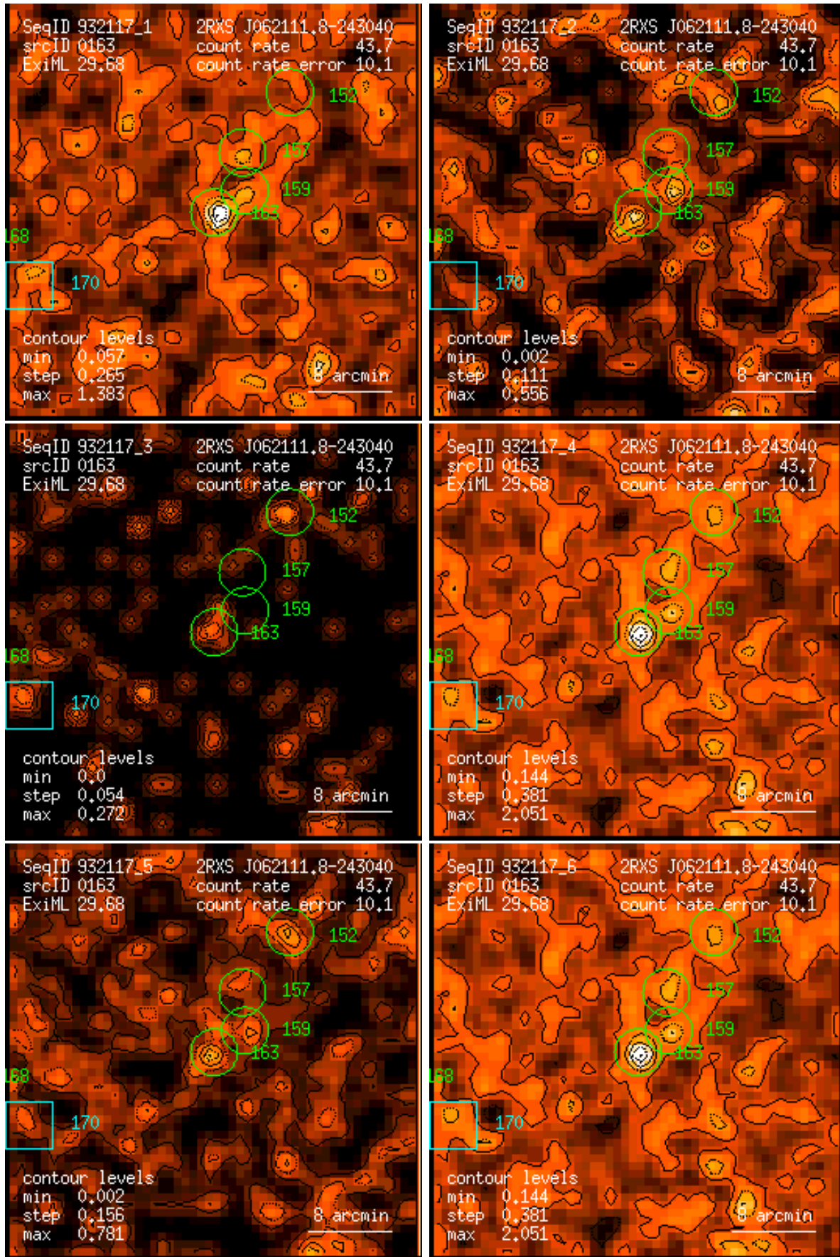
Figure 163: RASS 932117: detection 0163: band rate images, Gaussian filter: (1) PSPC channels 11 – 41, (2) 52 – 90, (3) 91 – 201, (4) 11 – 235, (5) 52 – 201, (6) 11 – 201. Broad band rates in counts/ks. Band rate contour levels in counts/ks/arcmin 2 .
