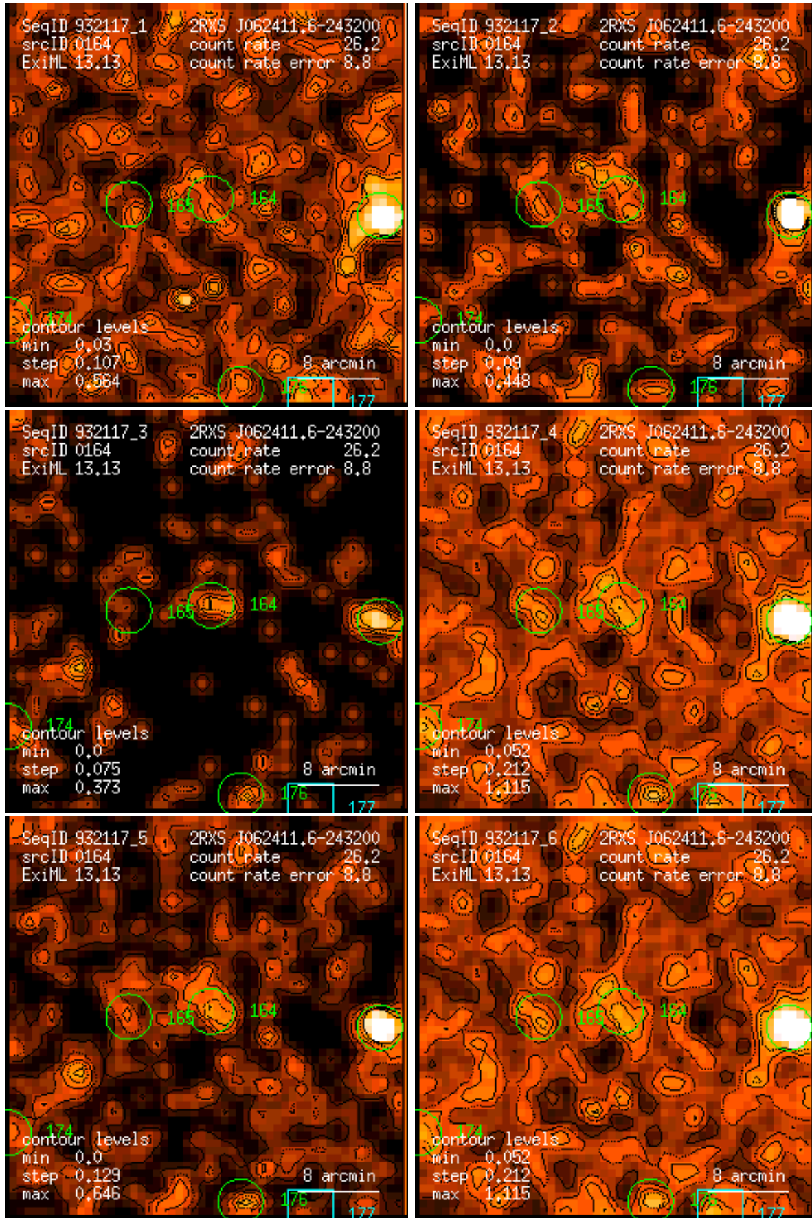
Figure 164: RASS 932117: detection 0164: band rate images, Gaussian filter: (1) PSPC channels 11 – 41, (2) 52 – 90, (3) 91 – 201, (4) 11 – 235, (5) 52 – 201, (6) 11 – 201. Broad band rates in counts/ks. Band rate contour levels in counts/ks/arcmin 2 .
