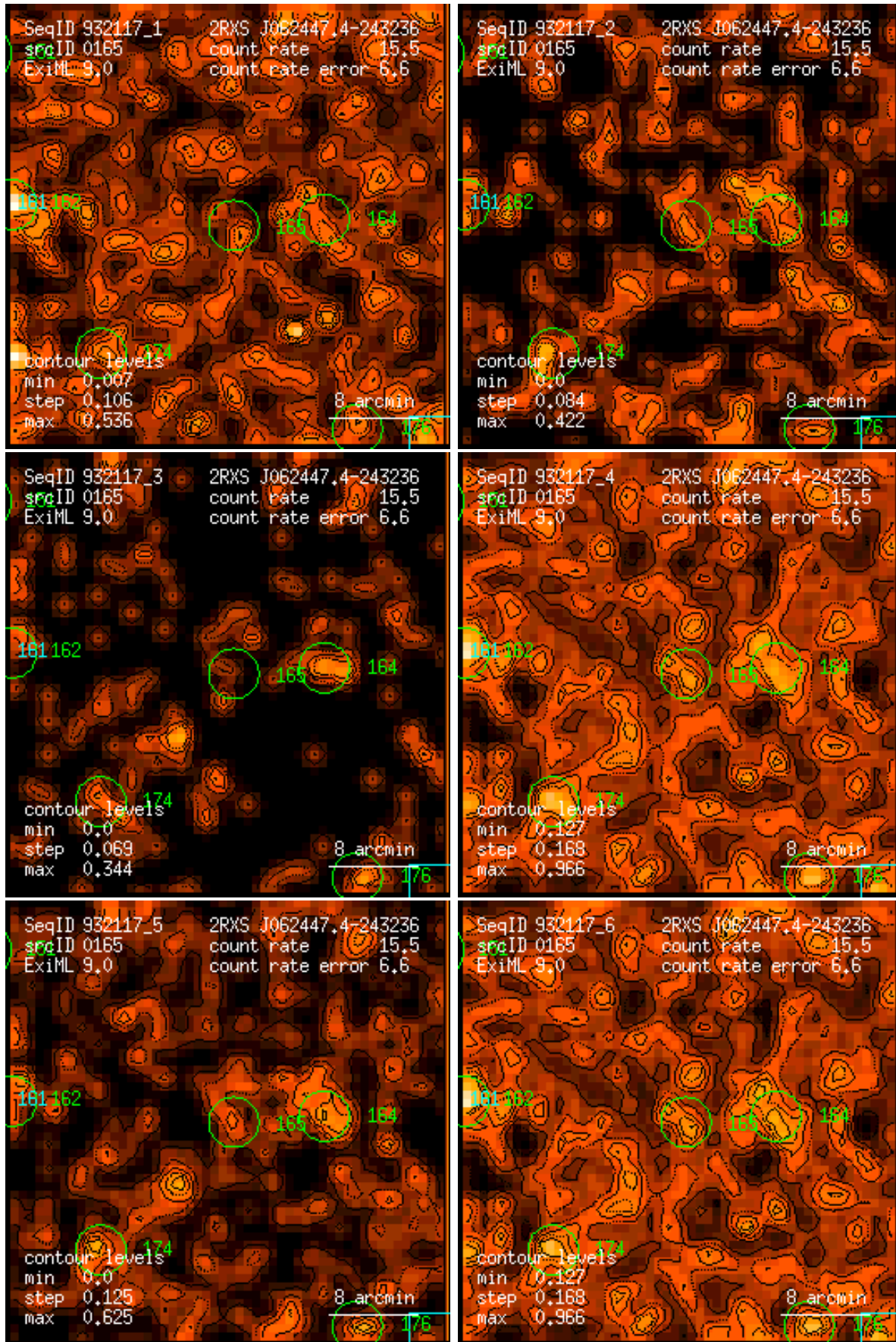
Figure 165: RASS 932117: detection 0165: band rate images, Gaussian filter: (1) PSPC channels 11 – 41, (2) 52 – 90, (3) 91 – 201, (4) 11 – 235, (5) 52 – 201, (6) 11 – 201. Broad band rates in counts/ks. Band rate contour levels in counts/ks/arcmin 2 .
