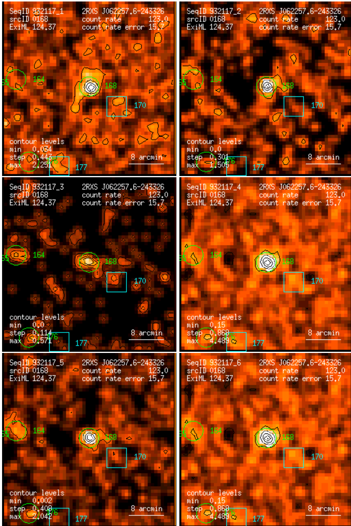
Figure 168: RASS 932117: detection 0168: band rate images, Gaussian filter: (1) PSPC channels 11 – 41, (2) 52 – 90, (3) 91 – 201, (4) 11 – 235, (5) 52 – 201, (6) 11 – 201. Broad band rates in counts/ks. Band rate contour levels in counts/ks/arcmin 2 .
