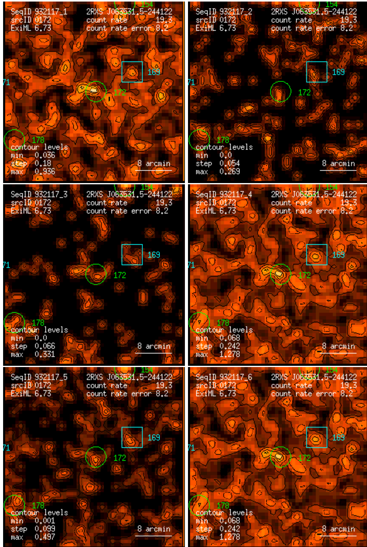
Figure 172: RASS 932117: detection 0172: band rate images, Gaussian filter: (1) PSPC channels 11 – 41, (2) 52 – 90, (3) 91 – 201, (4) 11 – 235, (5) 52 – 201, (6) 11 – 201. Broad band rates in counts/ks. Band rate contour levels in counts/ks/arcmin 2 .
