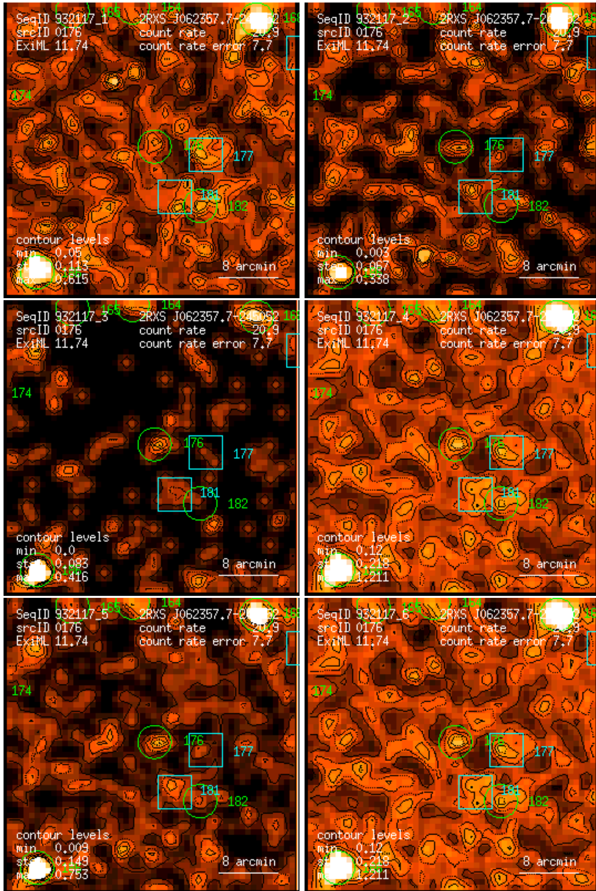
Figure 176: RASS 932117: detection 0176: band rate images, Gaussian filter: (1) PSPC channels 11 – 41, (2) 52 – 90, (3) 91 – 201, (4) 11 – 235, (5) 52 – 201, (6) 11 – 201. Broad band rates in counts/ks. Band rate contour levels in counts/ks/arcmin 2 .
