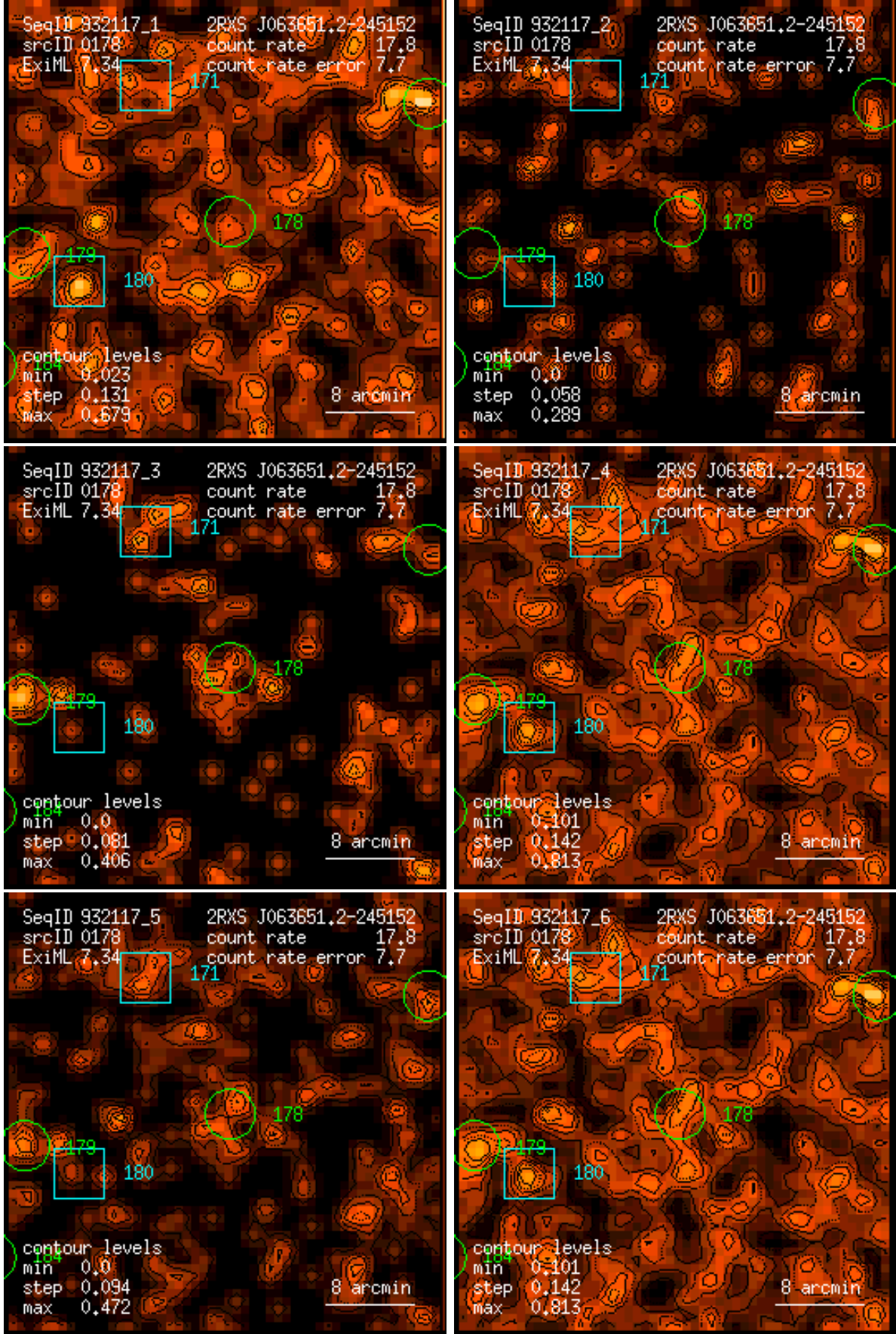
Figure 178: RASS 932117: detection 0178: band rate images, Gaussian filter: (1) PSPC channels 11 – 41, (2) 52 – 90, (3) 91 – 201, (4) 11 – 235, (5) 52 – 201, (6) 11 – 201. Broad band rates in counts/ks. Band rate contour levels in counts/ks/arcmin 2 .
