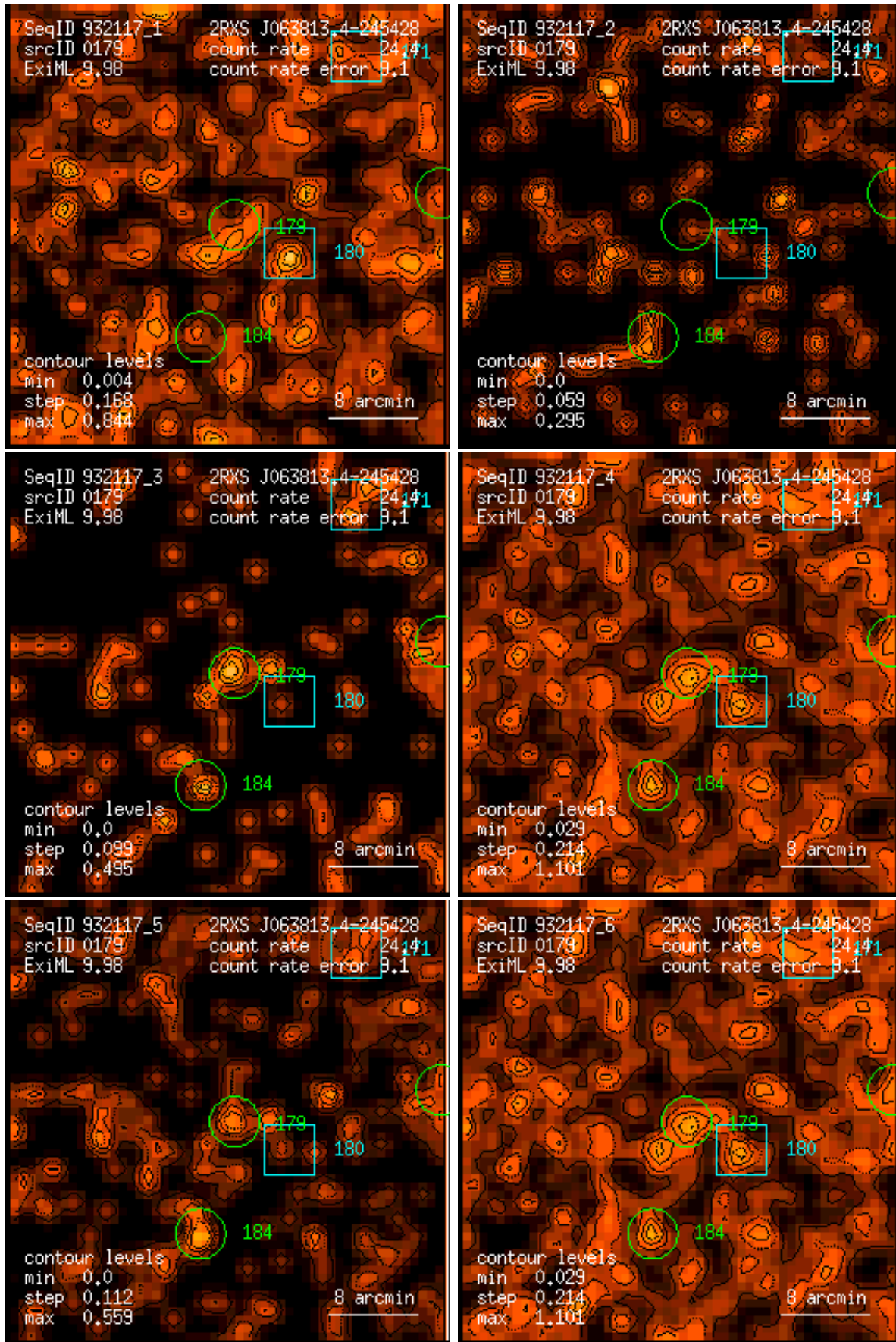
Figure 179: RASS 932117: detection 0179: band rate images, Gaussian filter: (1) PSPC channels 11 – 41, (2) 52 – 90, (3) 91 – 201, (4) 11 – 235, (5) 52 – 201, (6) 11 – 201. Broad band rates in counts/ks. Band rate contour levels in counts/ks/arcmin 2 .
