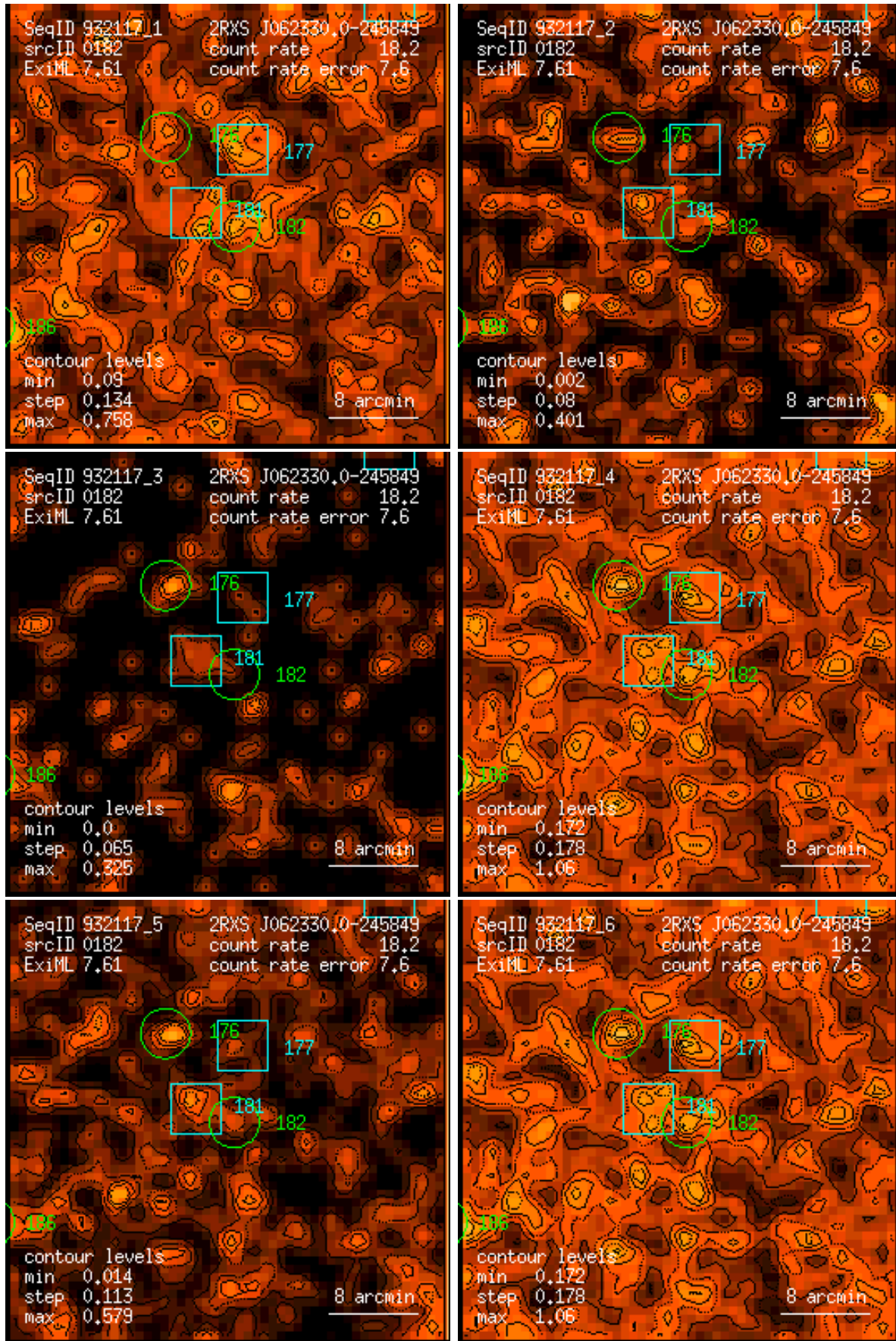
Figure 182: RASS 932117: detection 0182: band rate images, Gaussian filter: (1) PSPC channels 11 – 41, (2) 52 – 90, (3) 91 – 201, (4) 11 – 235, (5) 52 – 201, (6) 11 – 201. Broad band rates in counts/ks. Band rate contour levels in counts/ks/arcmin 2 .
