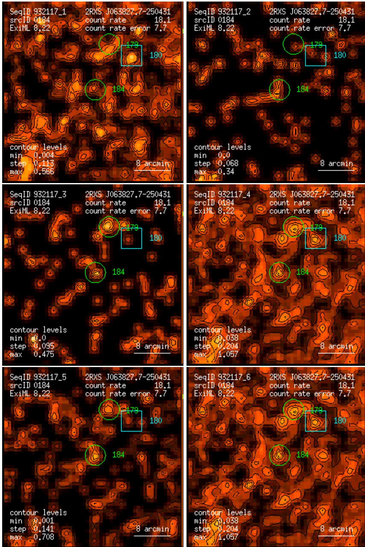
Figure 184: RASS 932117: detection 0184: band rate images, Gaussian filter: (1) PSPC channels 11 – 41, (2) 52 – 90, (3) 91 – 201, (4) 11 – 235, (5) 52 – 201, (6) 11 – 201. Broad band rates in counts/ks. Band rate contour levels in counts/ks/arcmin 2 .
