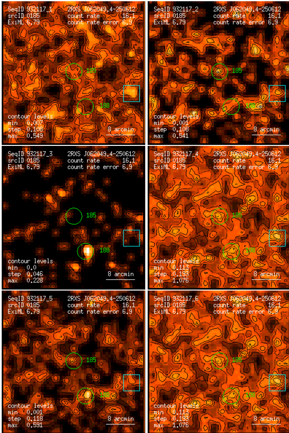
Figure 185: RASS 932117: detection 0185: band rate images, Gaussian filter: (1) PSPC channels 11 – 41, (2) 52 – 90, (3) 91 – 201, (4) 11 – 235, (5) 52 – 201, (6) 11 – 201. Broad band rates in counts/ks. Band rate contour levels in counts/ks/arcmin 2 .
