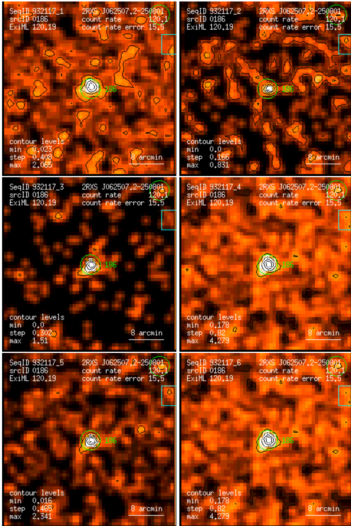
Figure 186: RASS 932117: detection 0186: band rate images, Gaussian filter: (1) PSPC channels 11 – 41, (2) 52 – 90, (3) 91 – 201, (4) 11 – 235, (5) 52 – 201, (6) 11 – 201. Broad band rates in counts/ks. Band rate contour levels in counts/ks/arcmin 2 .
