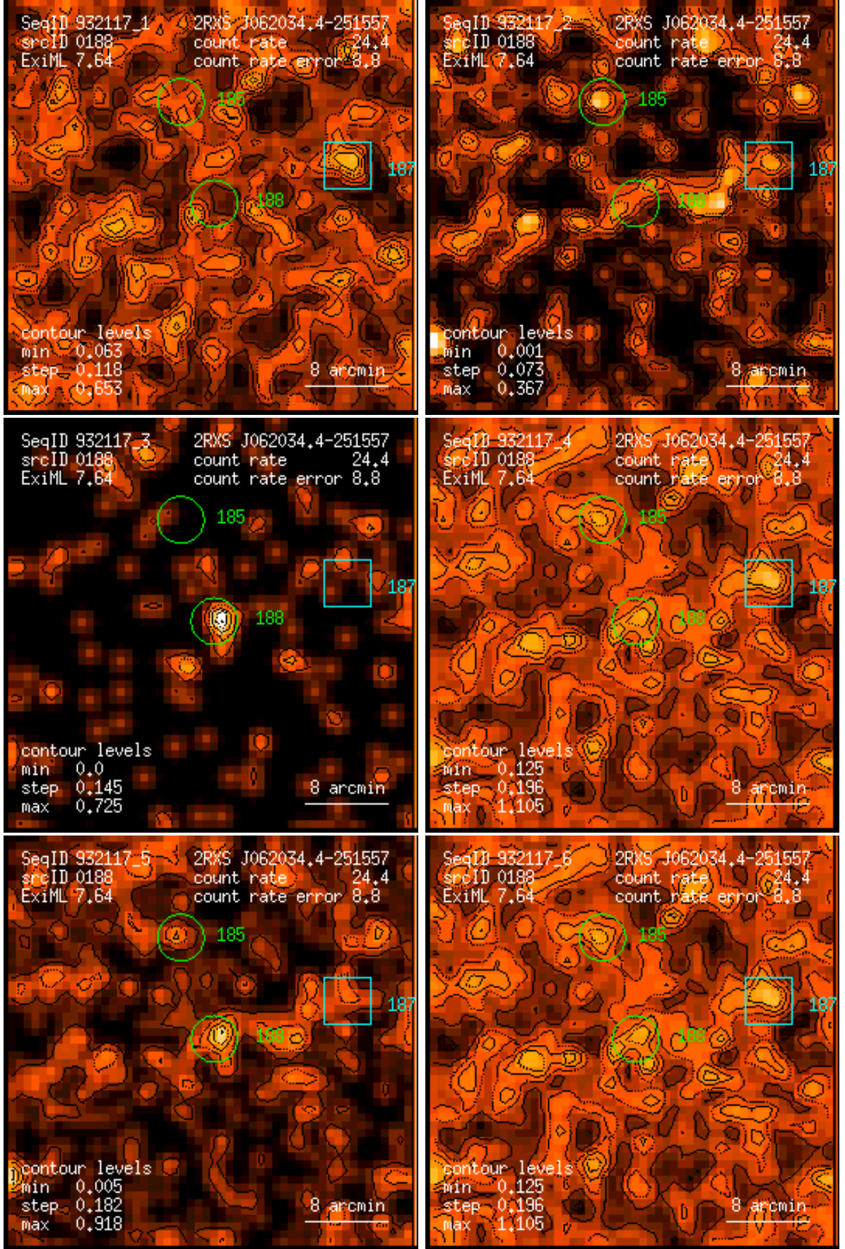
Figure 188: RASS 932117: detection 0188: band rate images, Gaussian filter: (1) PSPC channels 11 – 41, (2) 52 – 90, (3) 91 – 201, (4) 11 – 235, (5) 52 – 201, (6) 11 – 201. Broad band rates in counts/ks. Band rate contour levels in counts/ks/arcmin 2 .
