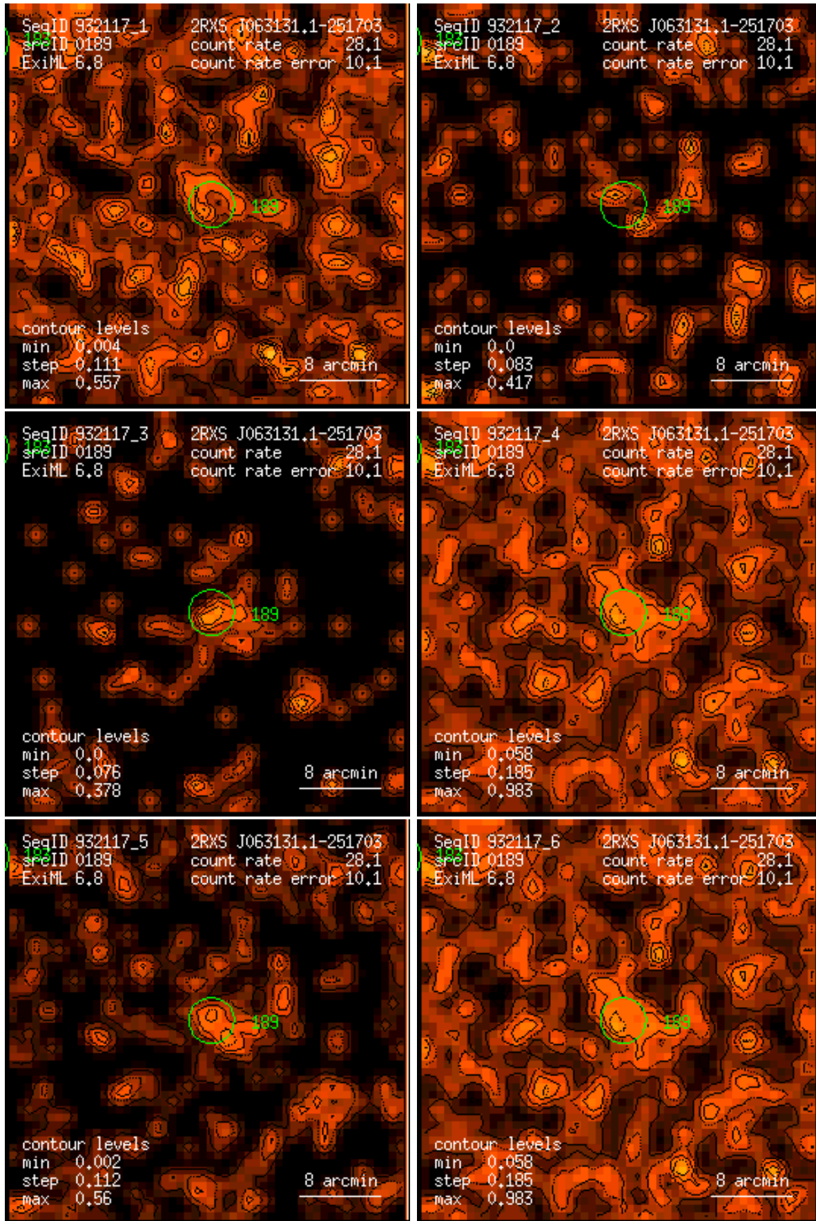
Figure 189: RASS 932117: detection 0189: band rate images, Gaussian filter: (1) PSPC channels 11 – 41, (2) 52 – 90, (3) 91 – 201, (4) 11 – 235, (5) 52 – 201, (6) 11 – 201. Broad band rates in counts/ks. Band rate contour levels in counts/ks/arcmin 2 .
