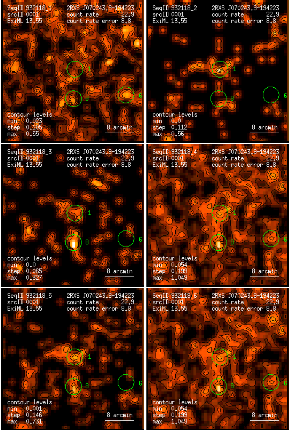
Figure 1: RASS 932118: detection 0001: band rate images, Gaussian filter: (1) PSPC channels 11 – 41, (2) 52 – 90, (3) 91 – 201, (4) 11 – 235, (5) 52 – 201, (6) 11 – 201. Broad band rates in counts/ks. Band rate contour levels in counts/ks/arcmin 2 .
