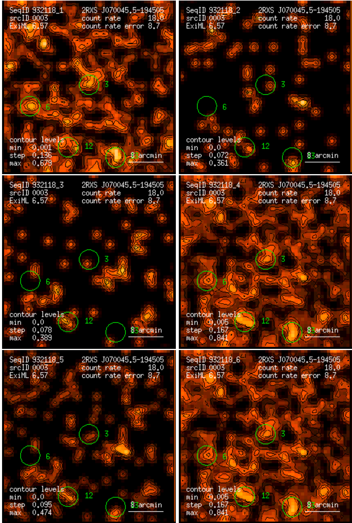
Figure 3: RASS 932118: detection 0003: band rate images, Gaussian filter: (1) PSPC channels 11 – 41, (2) 52 – 90, (3) 91 – 201, (4) 11 – 235, (5) 52 – 201, (6) 11 – 201. Broad band rates in counts/ks. Band rate contour levels in counts/ks/arcmin 2 .
