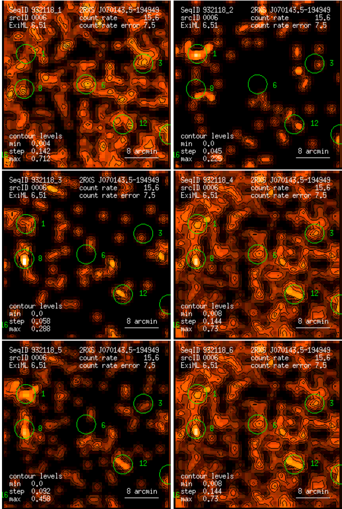
Figure 6: RASS 932118: detection 0006: band rate images, Gaussian filter: (1) PSPC channels 11 – 41, (2) 52 – 90, (3) 91 – 201, (4) 11 – 235, (5) 52 – 201, (6) 11 – 201. Broad band rates in counts/ks. Band rate contour levels in counts/ks/arcmin 2 .
