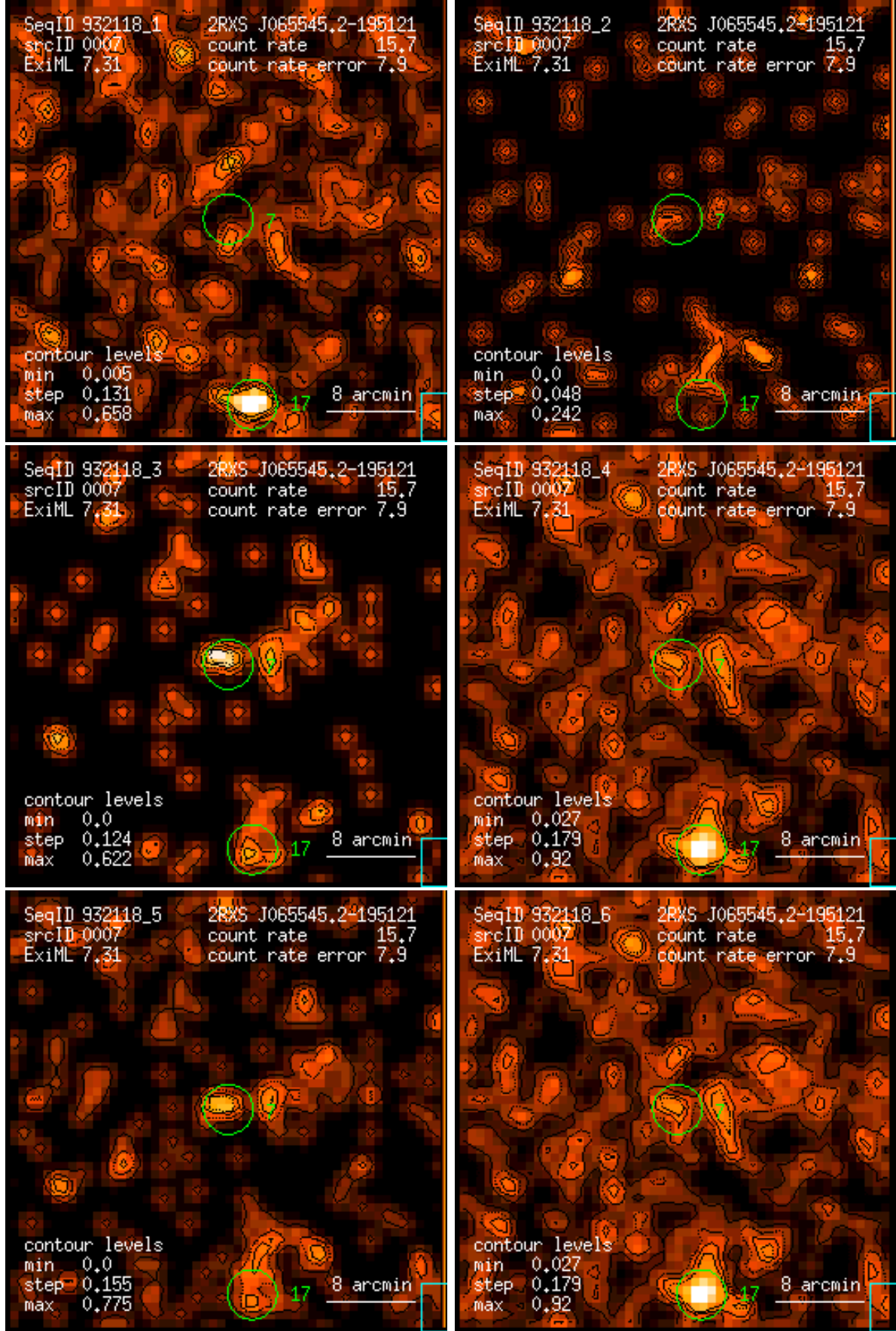
Figure 7: RASS 932118: detection 0007: band rate images, Gaussian filter: (1) PSPC channels 11 – 41, (2) 52 – 90, (3) 91 – 201, (4) 11 – 235, (5) 52 – 201, (6) 11 – 201. Broad band rates in counts/ks. Band rate contour levels in counts/ks/arcmin 2 .
