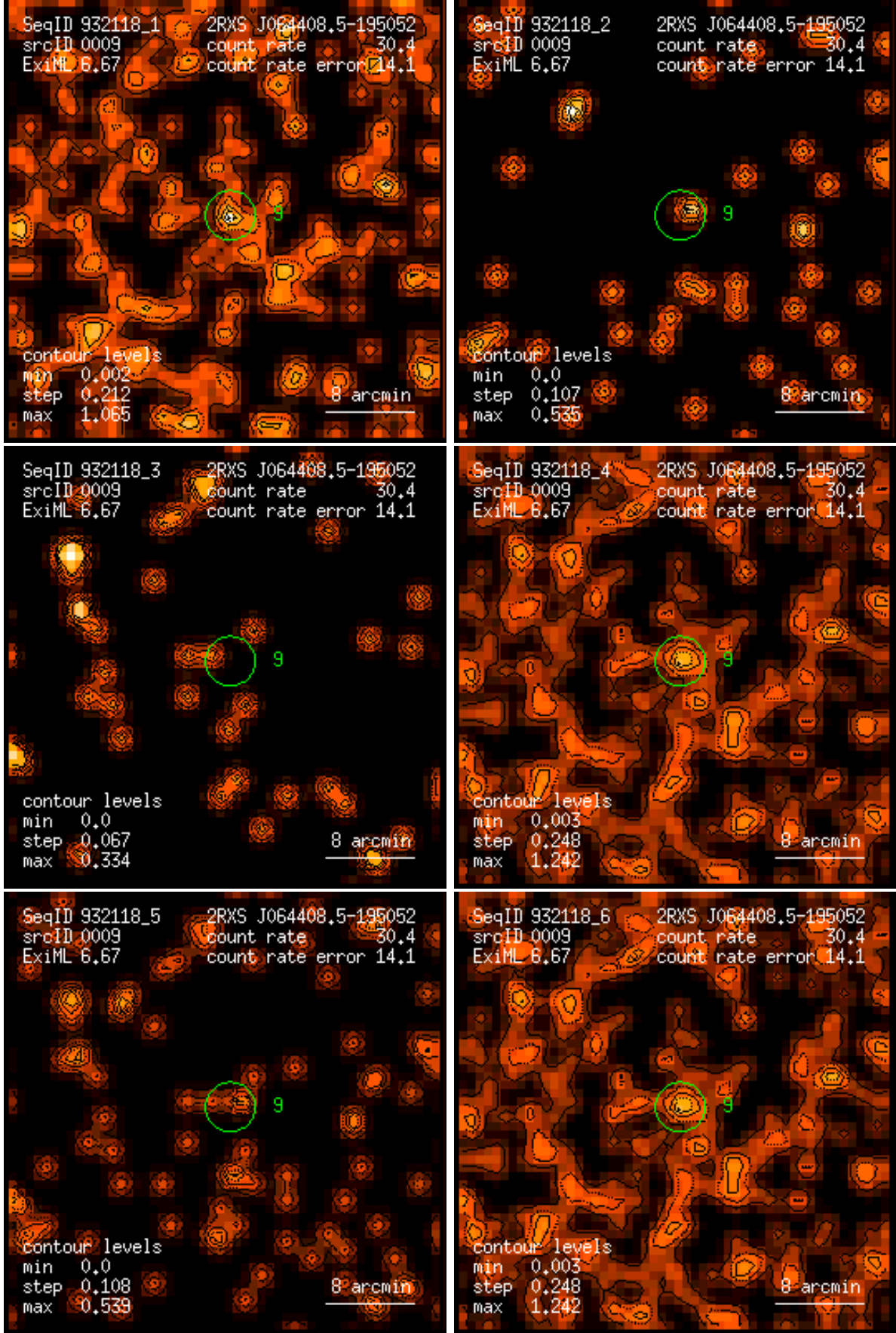
Figure 9: RASS 932118: detection 0009: band rate images, Gaussian filter: (1) PSPC channels 11 – 41, (2) 52 – 90, (3) 91 – 201, (4) 11 – 235, (5) 52 – 201, (6) 11 – 201. Broad band rates in counts/ks. Band rate contour levels in counts/ks/arcmin 2 .
