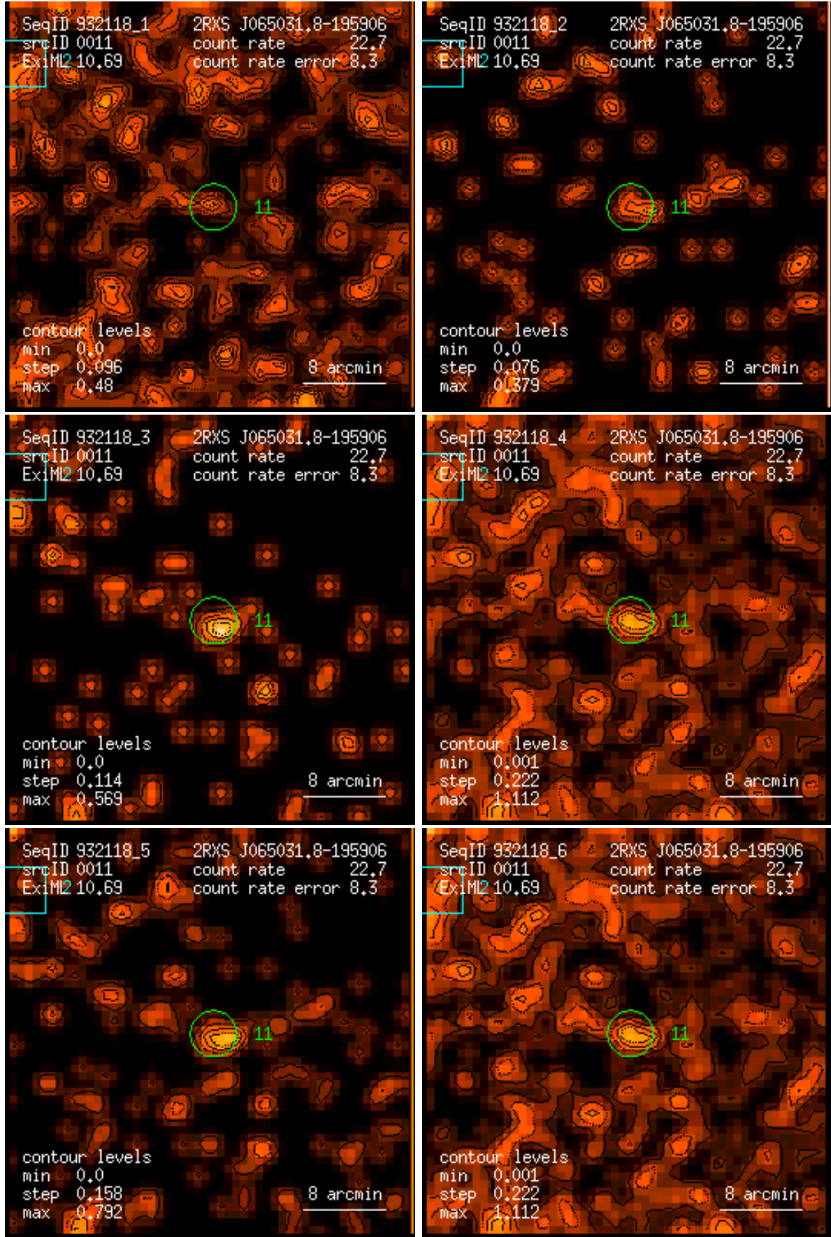
Figure 11: RASS 932118: detection 0011: band rate images, Gaussian filter: (1) PSPC channels 11 – 41, (2) 52 – 90, (3) 91 – 201, (4) 11 – 235, (5) 52 – 201, (6) 11 – 201. Broad band rates in counts/ks. Band rate contour levels in counts/ks/arcmin 2 .
