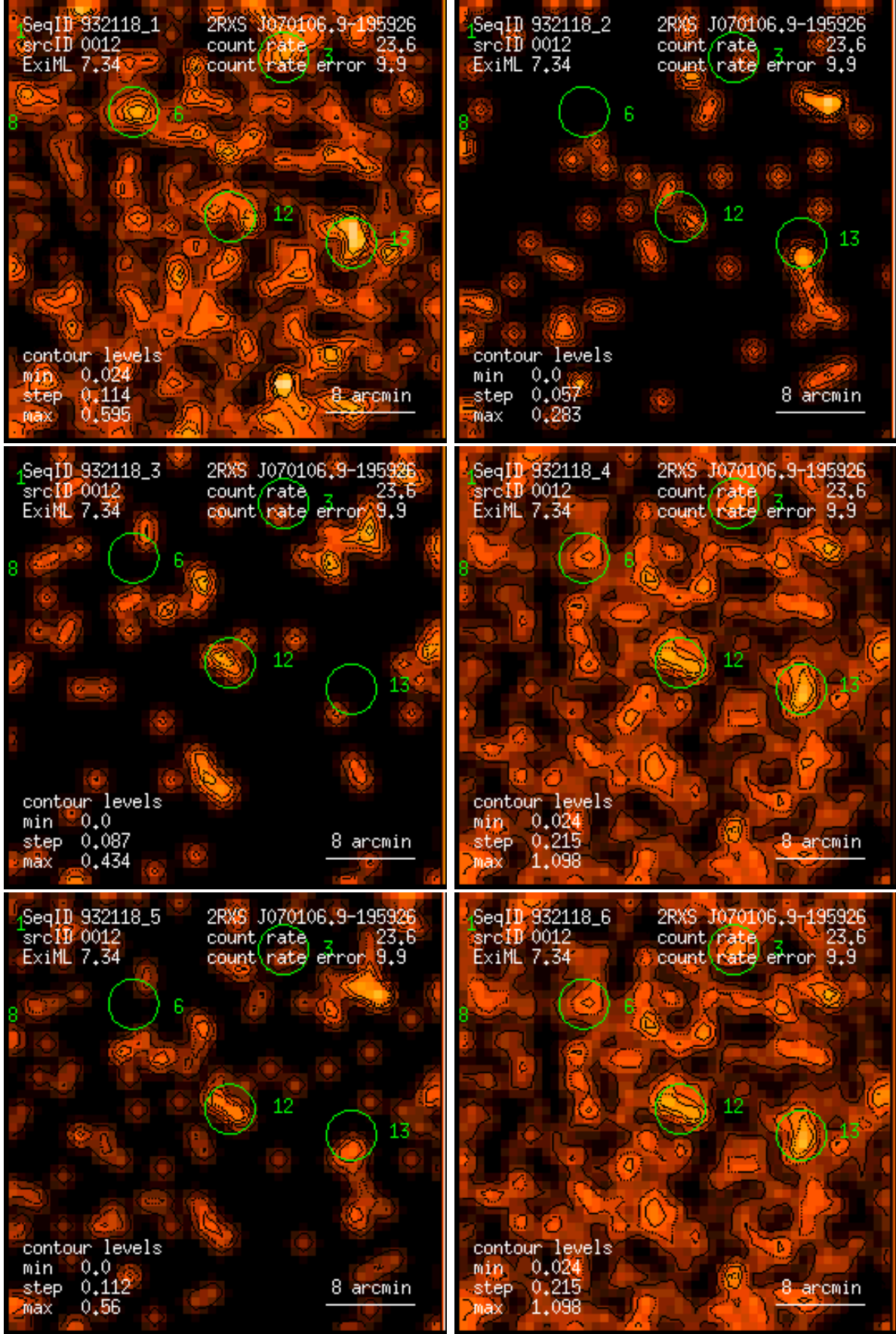
Figure 12: RASS 932118: detection 0012: band rate images, Gaussian filter: (1) PSPC channels 11 – 41, (2) 52 – 90, (3) 91 – 201, (4) 11 – 235, (5) 52 – 201, (6) 11 – 201. Broad band rates in counts/ks. Band rate contour levels in counts/ks/arcmin 2 .
