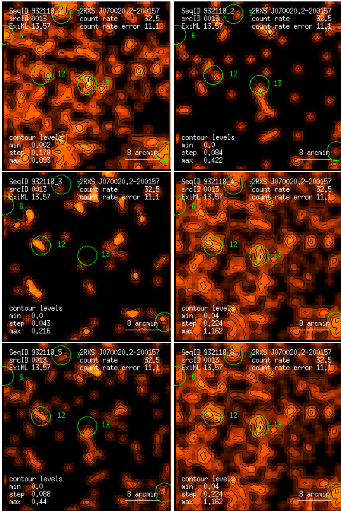
Figure 13: RASS 932118: detection 0013: band rate images, Gaussian filter: (1) PSPC channels 11 – 41, (2) 52 – 90, (3) 91 – 201, (4) 11 – 235, (5) 52 – 201, (6) 11 – 201. Broad band rates in counts/ks. Band rate contour levels in counts/ks/arcmin 2 .
