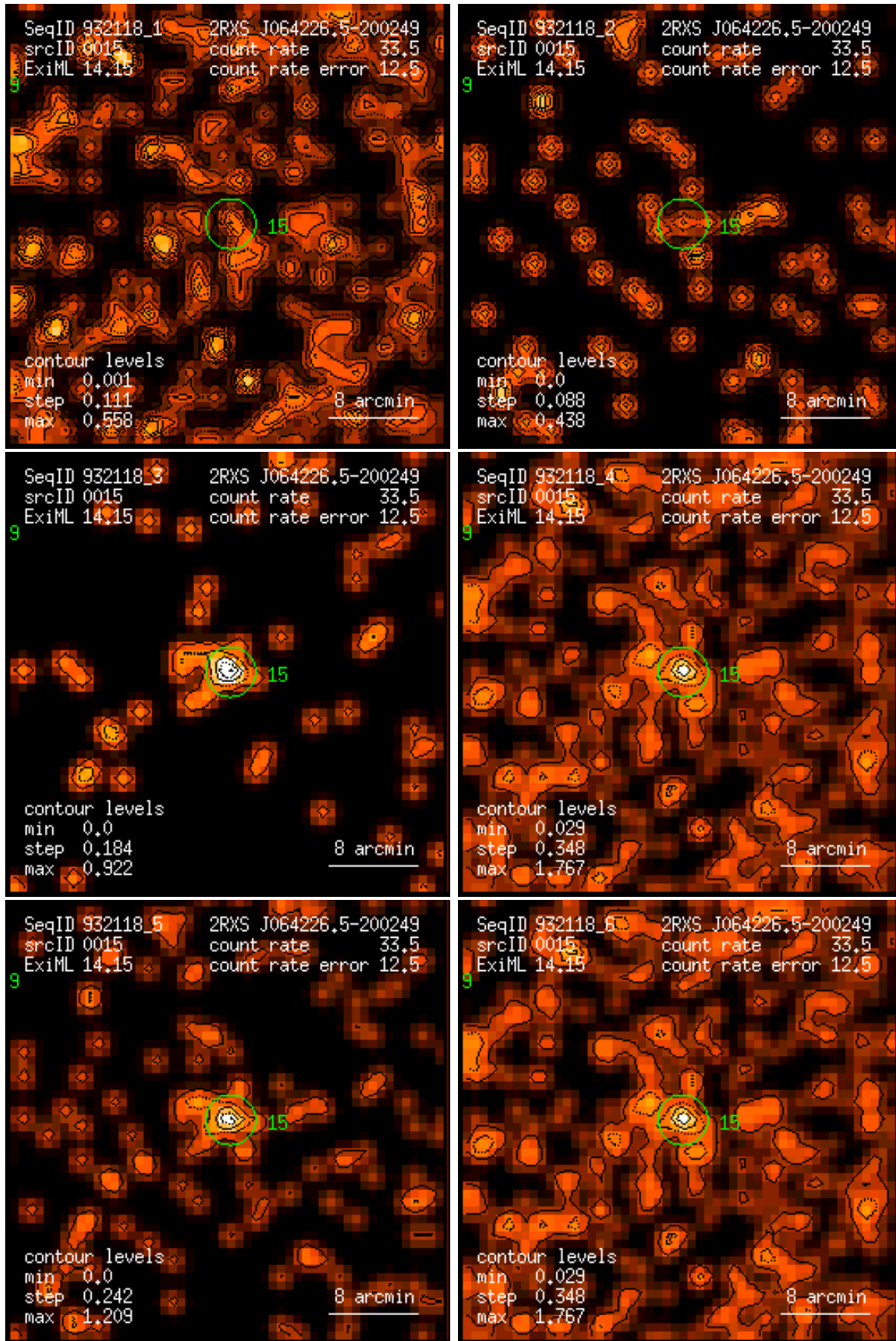
Figure 15: RASS 932118: detection 0015: band rate images, Gaussian filter: (1) PSPC channels 11 – 41, (2) 52 – 90, (3) 91 – 201, (4) 11 – 235, (5) 52 – 201, (6) 11 – 201. Broad band rates in counts/ks. Band rate contour levels in counts/ks/arcmin 2 .
