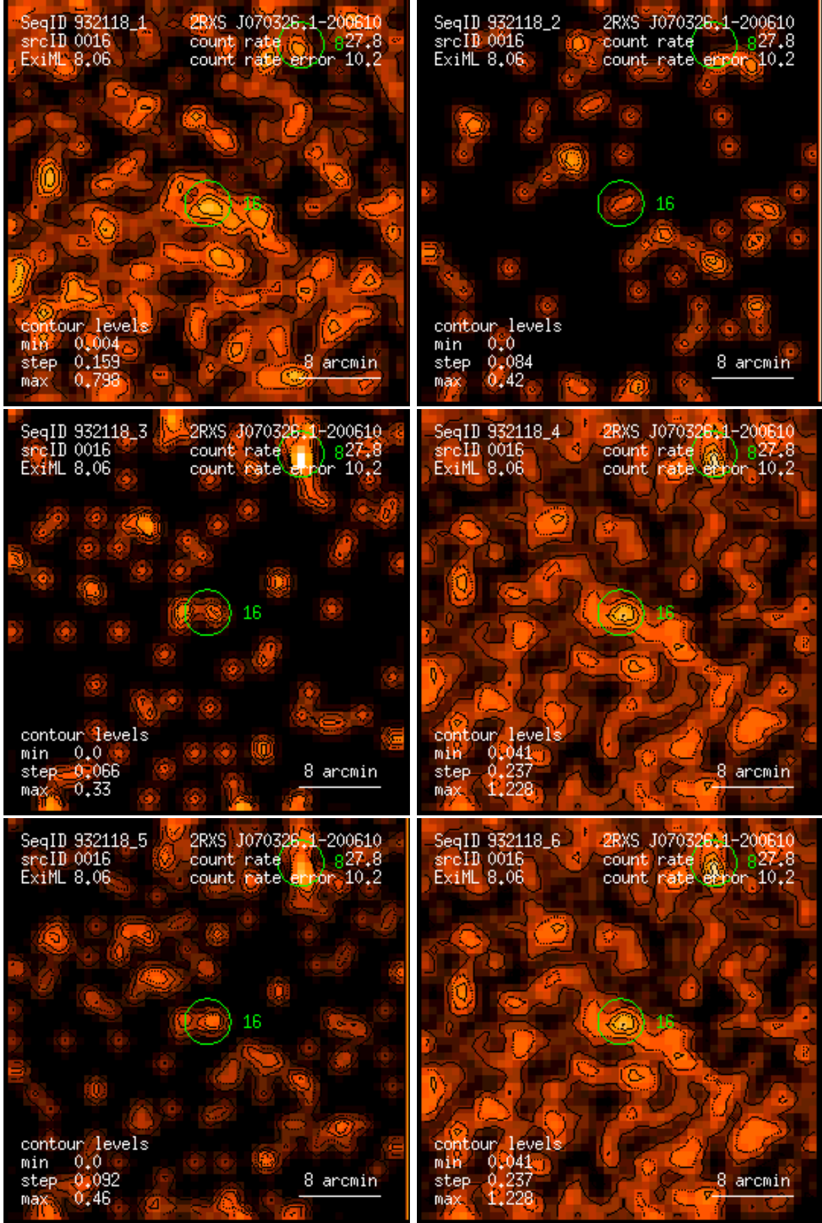
Figure 16: RASS 932118: detection 0016: band rate images, Gaussian filter: (1) PSPC channels 11 – 41, (2) 52 – 90, (3) 91 – 201, (4) 11 – 235, (5) 52 – 201, (6) 11 – 201. Broad band rates in counts/ks. Band rate contour levels in counts/ks/arcmin 2 .
