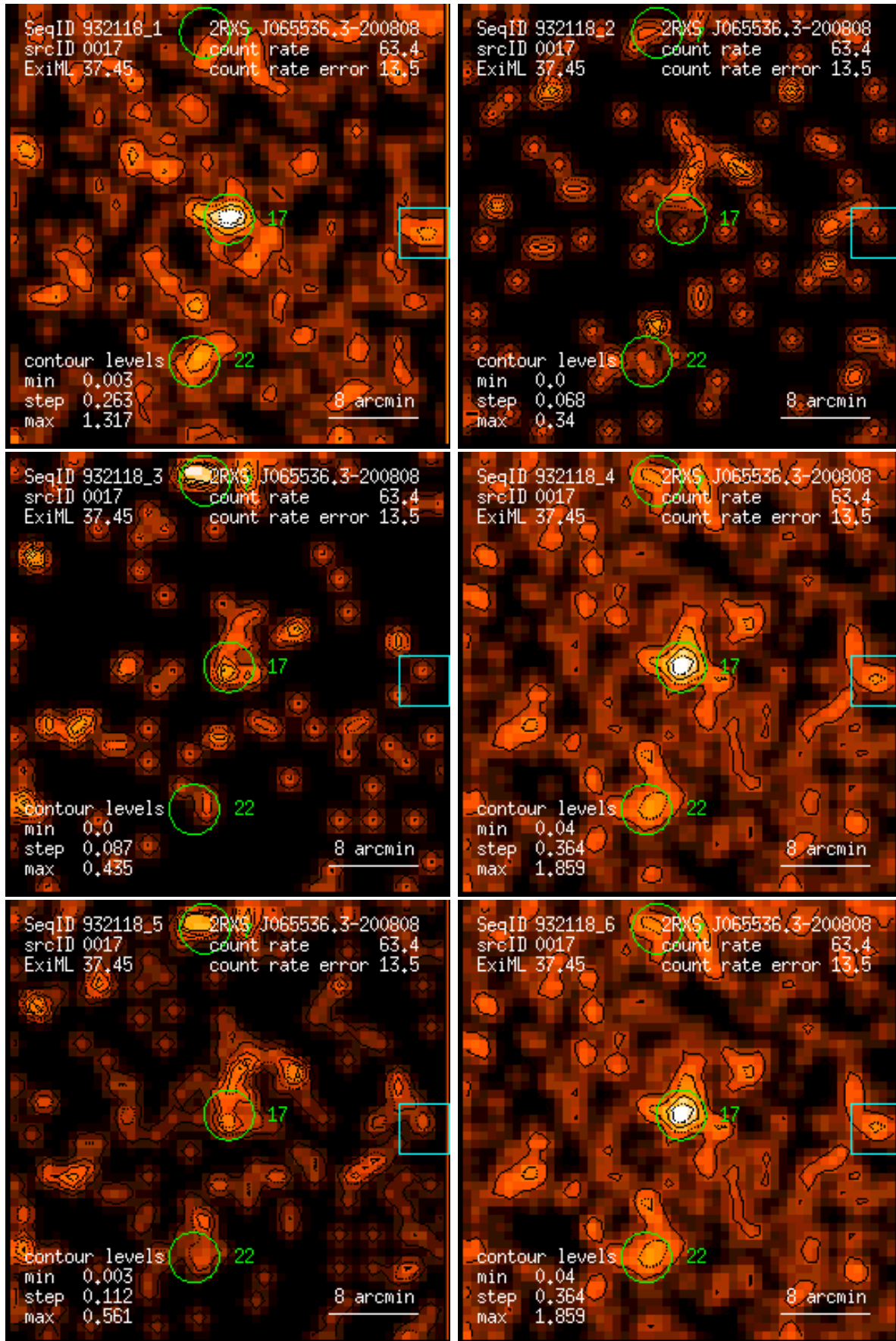
Figure 17: RASS 932118: detection 0017: band rate images, Gaussian filter: (1) PSPC channels 11 – 41, (2) 52 – 90, (3) 91 – 201, (4) 11 – 235, (5) 52 – 201, (6) 11 – 201. Broad band rates in counts/ks. Band rate contour levels in counts/ks/arcmin 2 .
