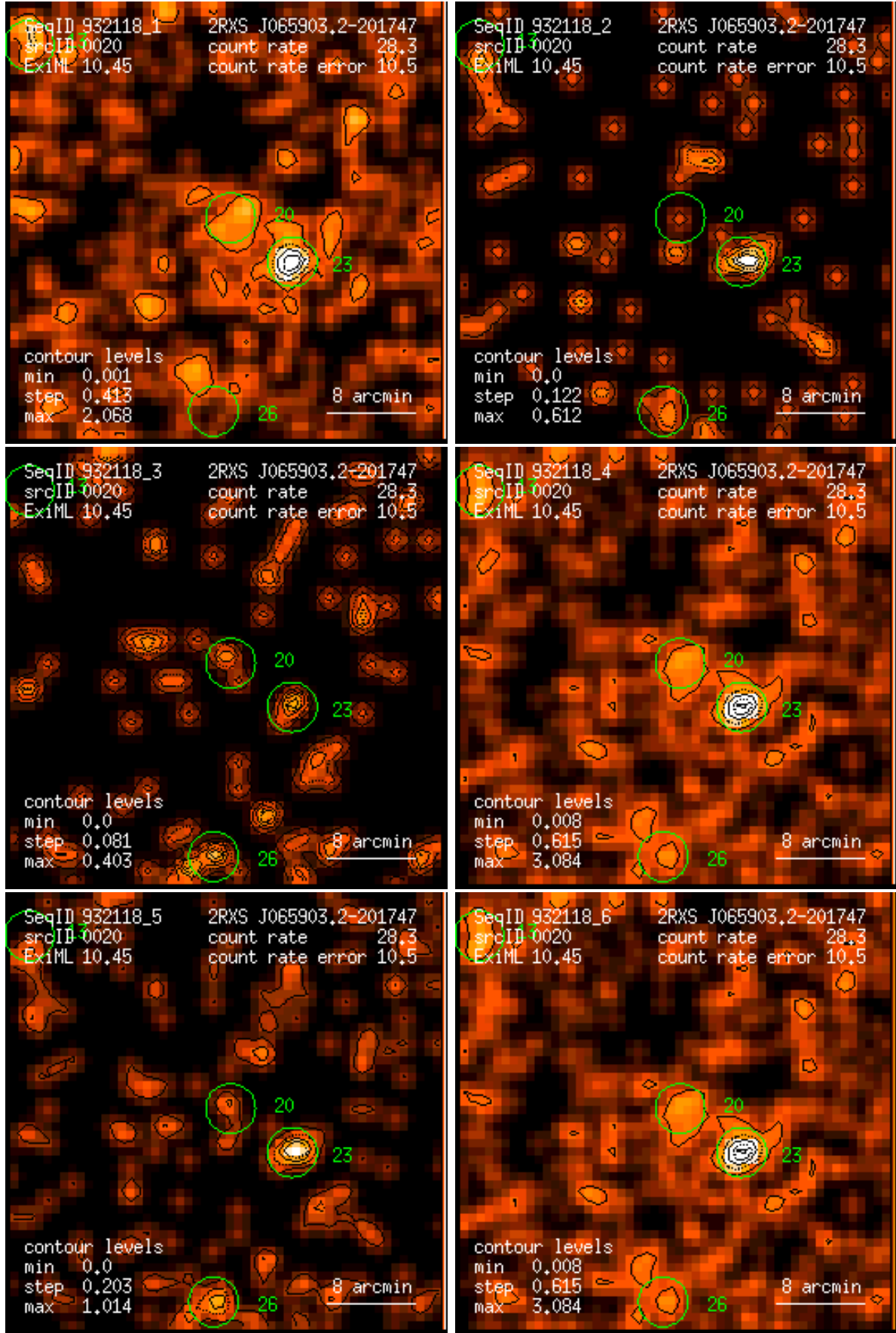
Figure 20: RASS 932118: detection 0020: band rate images, Gaussian filter: (1) PSPC channels 11 – 41, (2) 52 – 90, (3) 91 – 201, (4) 11 – 235, (5) 52 – 201, (6) 11 – 201. Broad band rates in counts/ks. Band rate contour levels in counts/ks/arcmin 2 .
