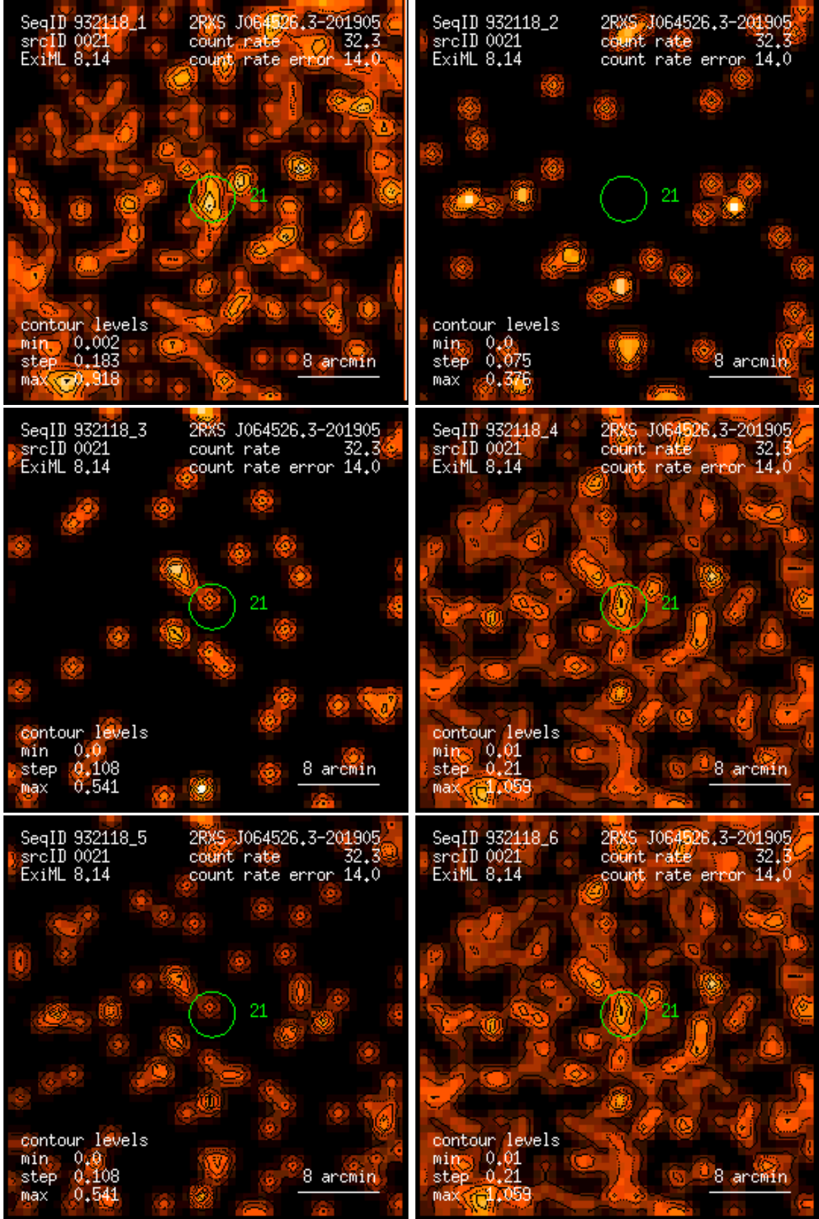
Figure 21: RASS 932118: detection 0021: band rate images, Gaussian filter: (1) PSPC channels 11 – 41, (2) 52 – 90, (3) 91 – 201, (4) 11 – 235, (5) 52 – 201, (6) 11 – 201. Broad band rates in counts/ks. Band rate contour levels in counts/ks/arcmin 2 .
