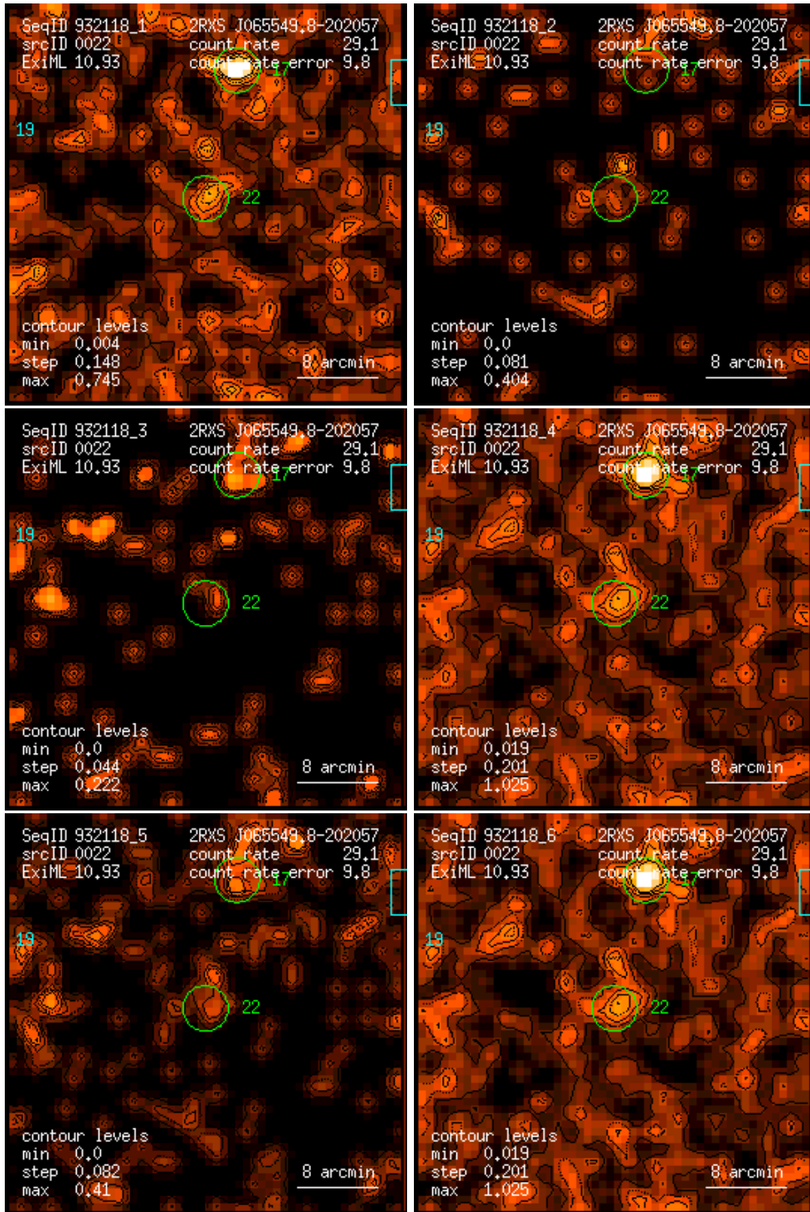
Figure 22: RASS 932118: detection 0022: band rate images, Gaussian filter: (1) PSPC channels 11 – 41, (2) 52 – 90, (3) 91 – 201, (4) 11 – 235, (5) 52 – 201, (6) 11 – 201. Broad band rates in counts/ks. Band rate contour levels in counts/ks/arcmin 2 .
