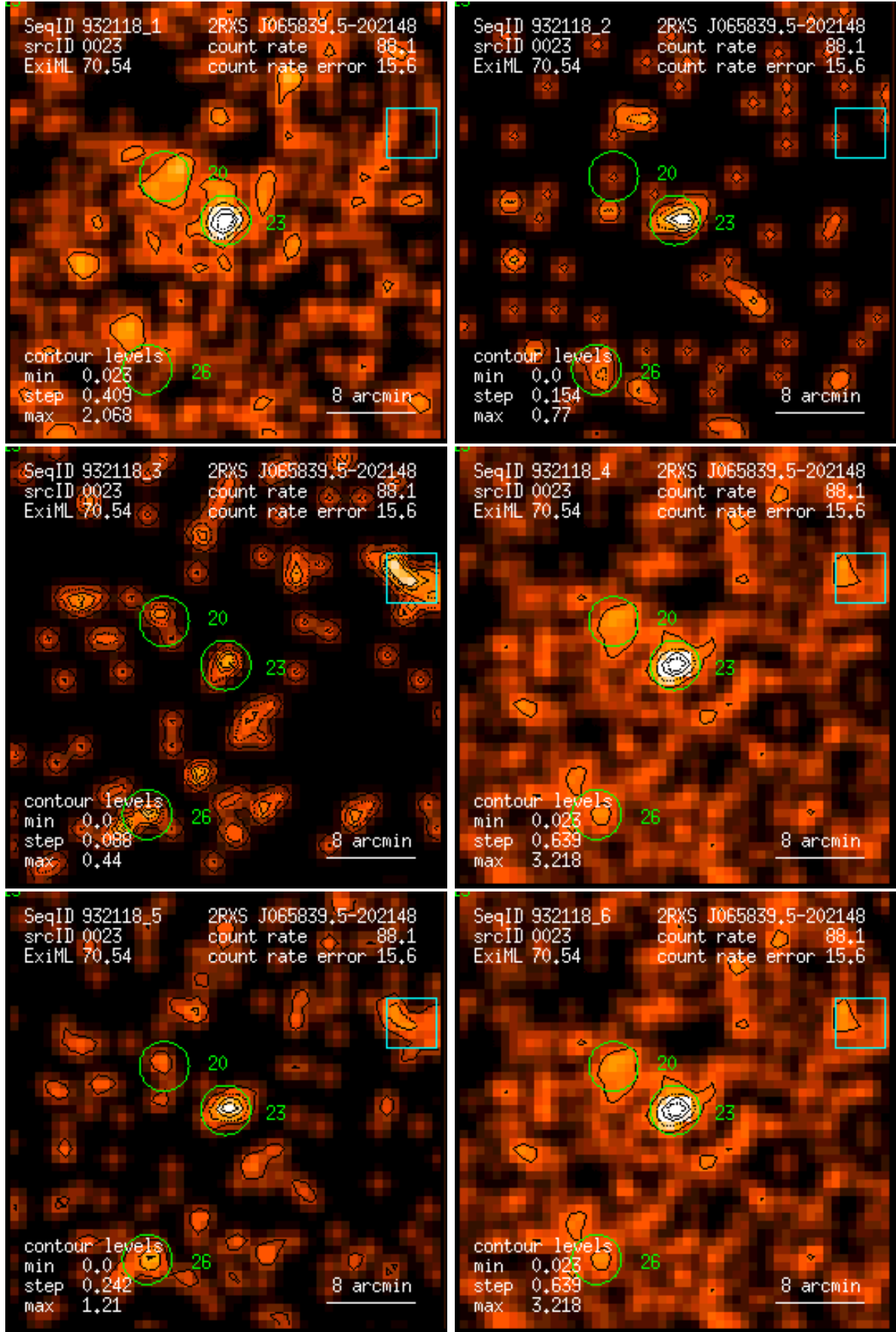
Figure 23: RASS 932118: detection 0023: band rate images, Gaussian filter: (1) PSPC channels 11 – 41, (2) 52 – 90, (3) 91 – 201, (4) 11 – 235, (5) 52 – 201, (6) 11 – 201. Broad band rates in counts/ks. Band rate contour levels in counts/ks/arcmin 2 .
