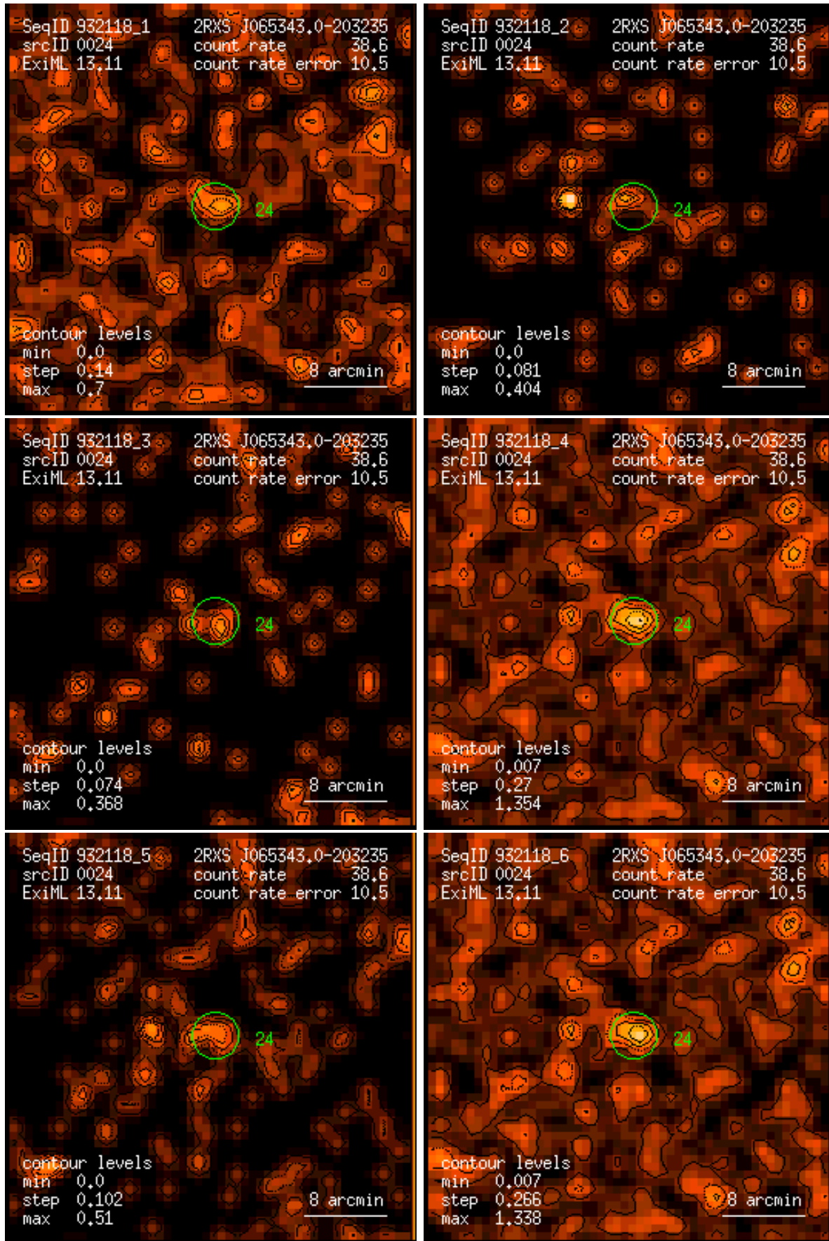
Figure 24: RASS 932118: detection 0024: band rate images, Gaussian filter: (1) PSPC channels 11 – 41, (2) 52 – 90, (3) 91 – 201, (4) 11 – 235, (5) 52 – 201, (6) 11 – 201. Broad band rates in counts/ks. Band rate contour levels in counts/ks/arcmin 2 .
