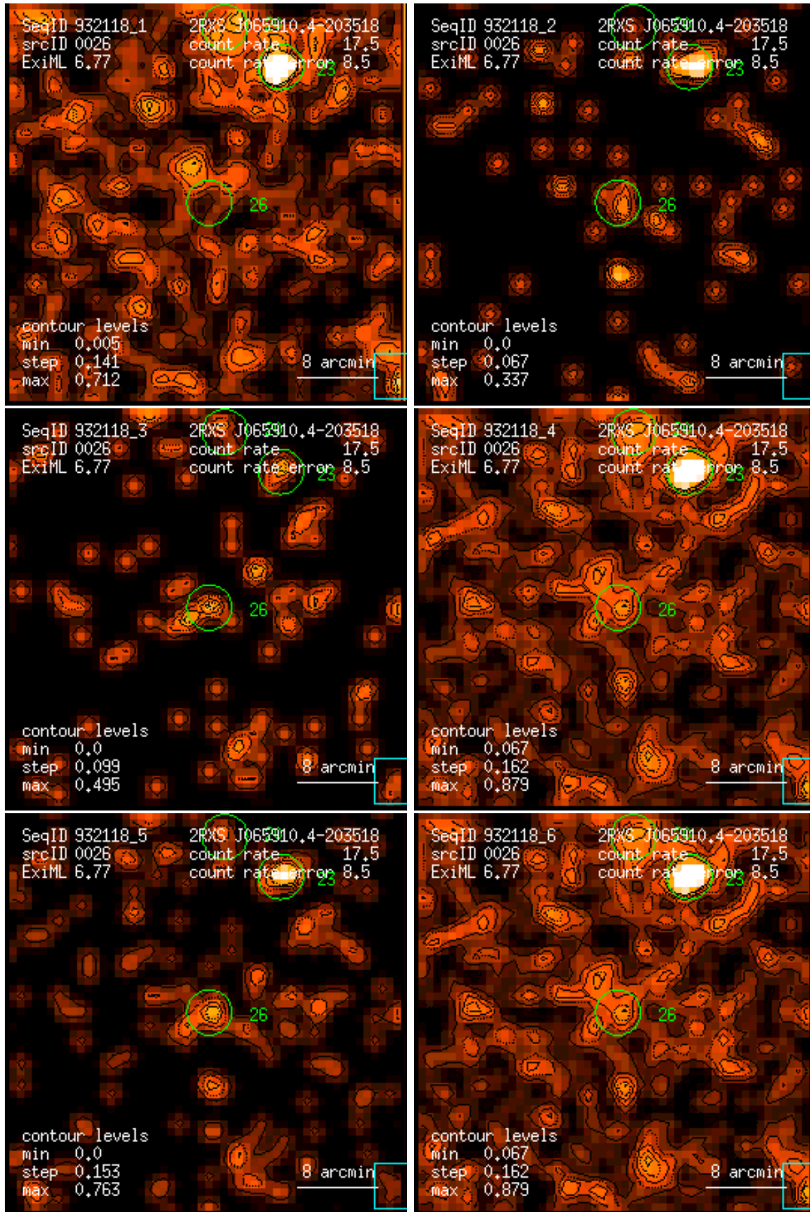
Figure 26: RASS 932118: detection 0026: band rate images, Gaussian filter: (1) PSPC channels 11 – 41, (2) 52 – 90, (3) 91 – 201, (4) 11 – 235, (5) 52 – 201, (6) 11 – 201. Broad band rates in counts/ks. Band rate contour levels in counts/ks/arcmin 2 .
