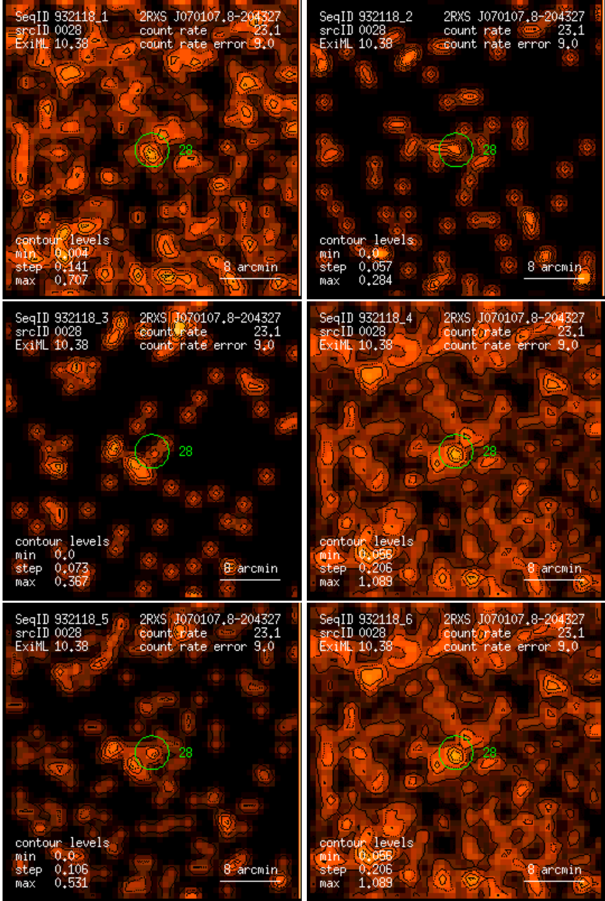
Figure 28: RASS 932118: detection 0028: band rate images, Gaussian filter: (1) PSPC channels 11 – 41, (2) 52 – 90, (3) 91 – 201, (4) 11 – 235, (5) 52 – 201, (6) 11 – 201. Broad band rates in counts/ks. Band rate contour levels in counts/ks/arcmin 2 .
