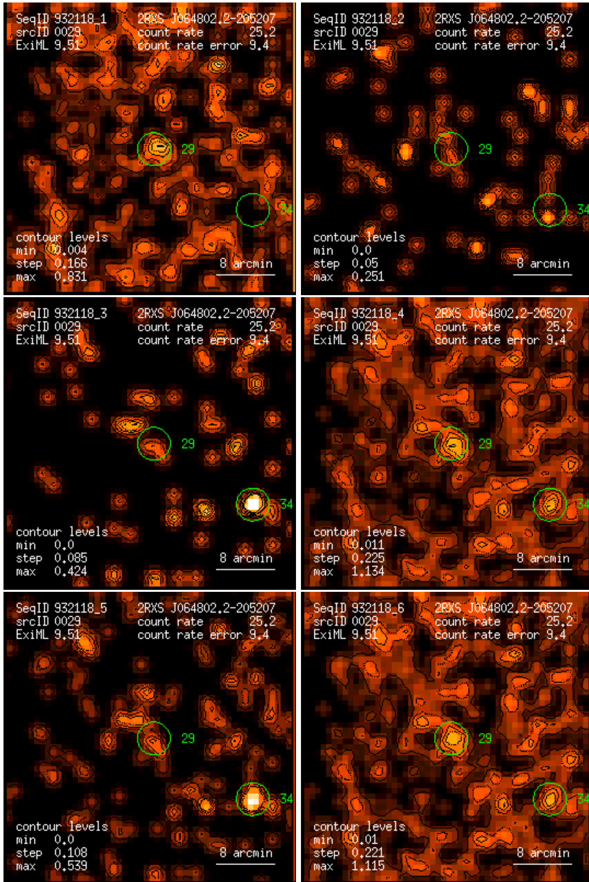
Figure 29: RASS 932118: detection 0029: band rate images, Gaussian filter: (1) PSPC channels 11 – 41, (2) 52 – 90, (3) 91 – 201, (4) 11 – 235, (5) 52 – 201, (6) 11 – 201. Broad band rates in counts/ks. Band rate contour levels in counts/ks/arcmin 2 .
