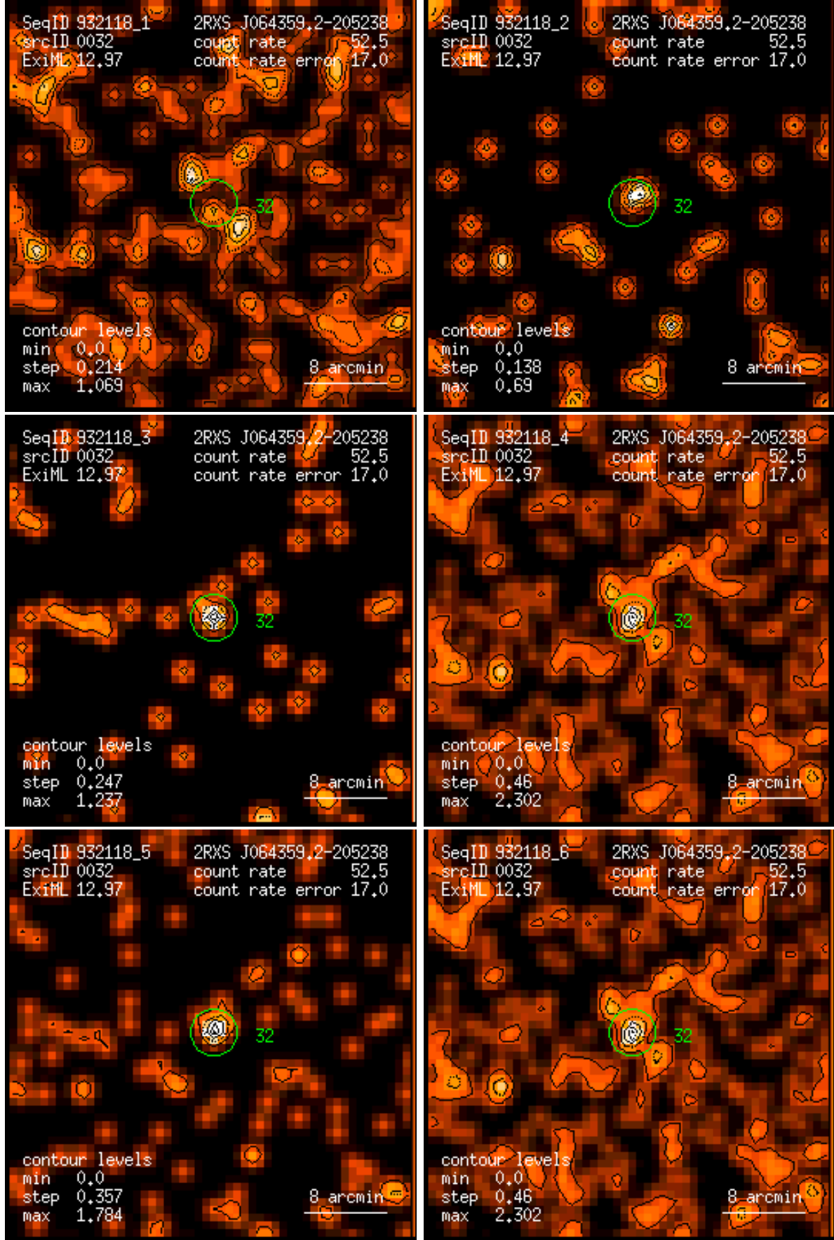
Figure 32: RASS 932118: detection 0032: band rate images, Gaussian filter: (1) PSPC channels 11 – 41, (2) 52 – 90, (3) 91 – 201, (4) 11 – 235, (5) 52 – 201, (6) 11 – 201. Broad band rates in counts/ks. Band rate contour levels in counts/ks/arcmin 2 .
