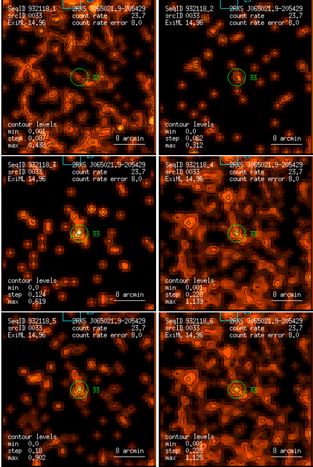
Figure 33: RASS 932118: detection 0033: band rate images, Gaussian filter: (1) PSPC channels 11 – 41, (2) 52 – 90, (3) 91 – 201, (4) 11 – 235, (5) 52 – 201, (6) 11 – 201. Broad band rates in counts/ks. Band rate contour levels in counts/ks/arcmin 2 .
