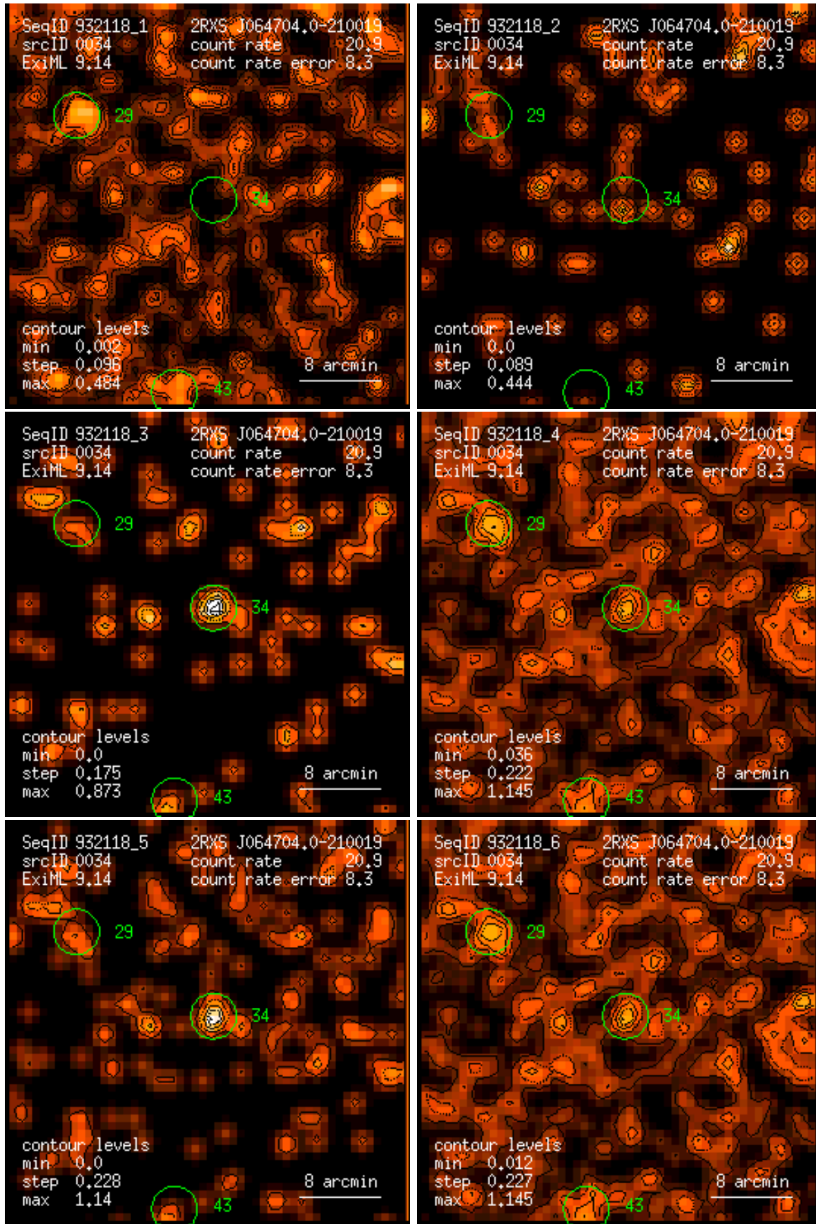
Figure 34: RASS 932118: detection 0034: band rate images, Gaussian filter: (1) PSPC channels 11 – 41, (2) 52 – 90, (3) 91 – 201, (4) 11 – 235, (5) 52 – 201, (6) 11 – 201. Broad band rates in counts/ks. Band rate contour levels in counts/ks/arcmin 2 .
