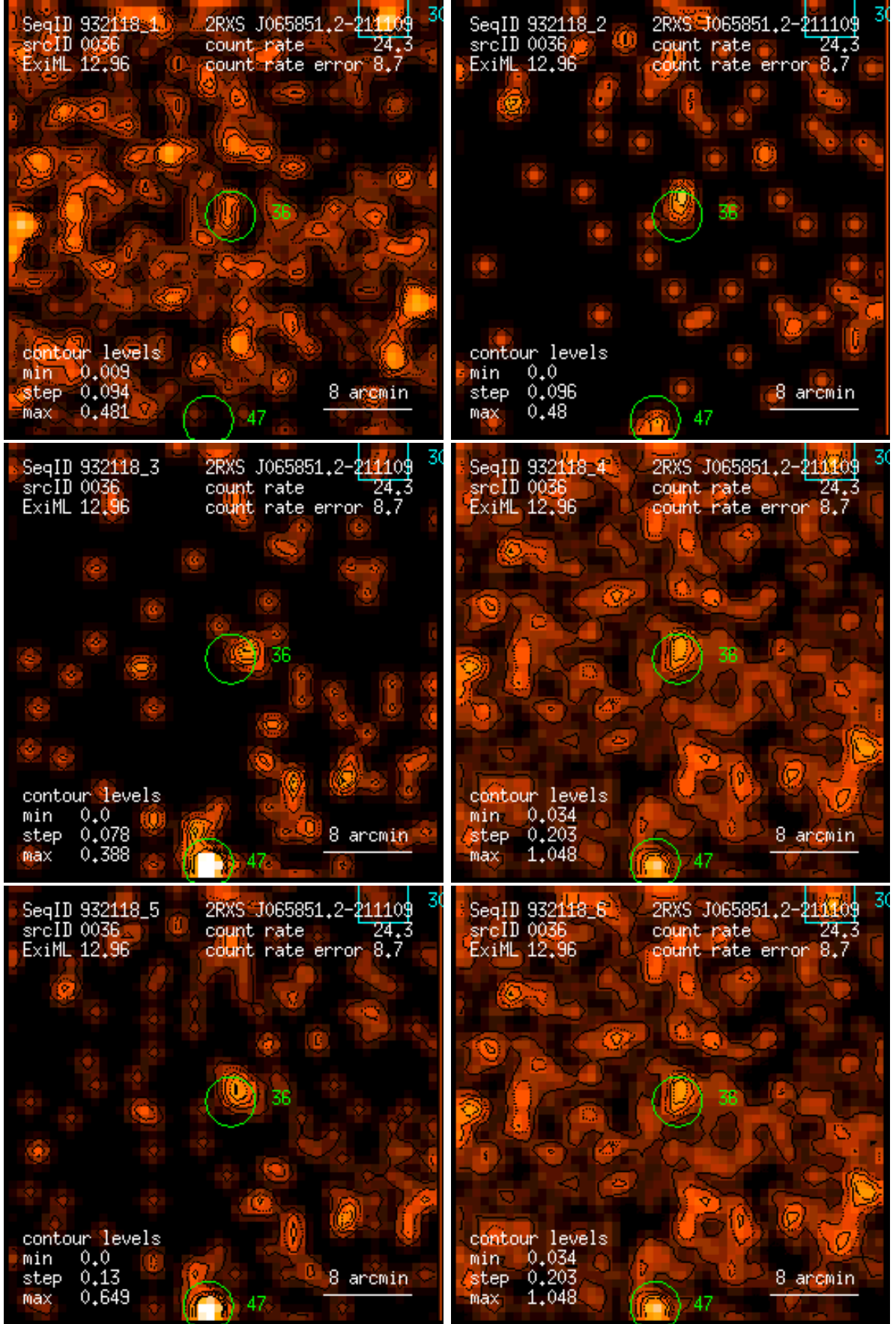
Figure 36: RASS 932118: detection 0036: band rate images, Gaussian filter: (1) PSPC channels 11 – 41, (2) 52 – 90, (3) 91 – 201, (4) 11 – 235, (5) 52 – 201, (6) 11 – 201. Broad band rates in counts/ks. Band rate contour levels in counts/ks/arcmin 2 .
