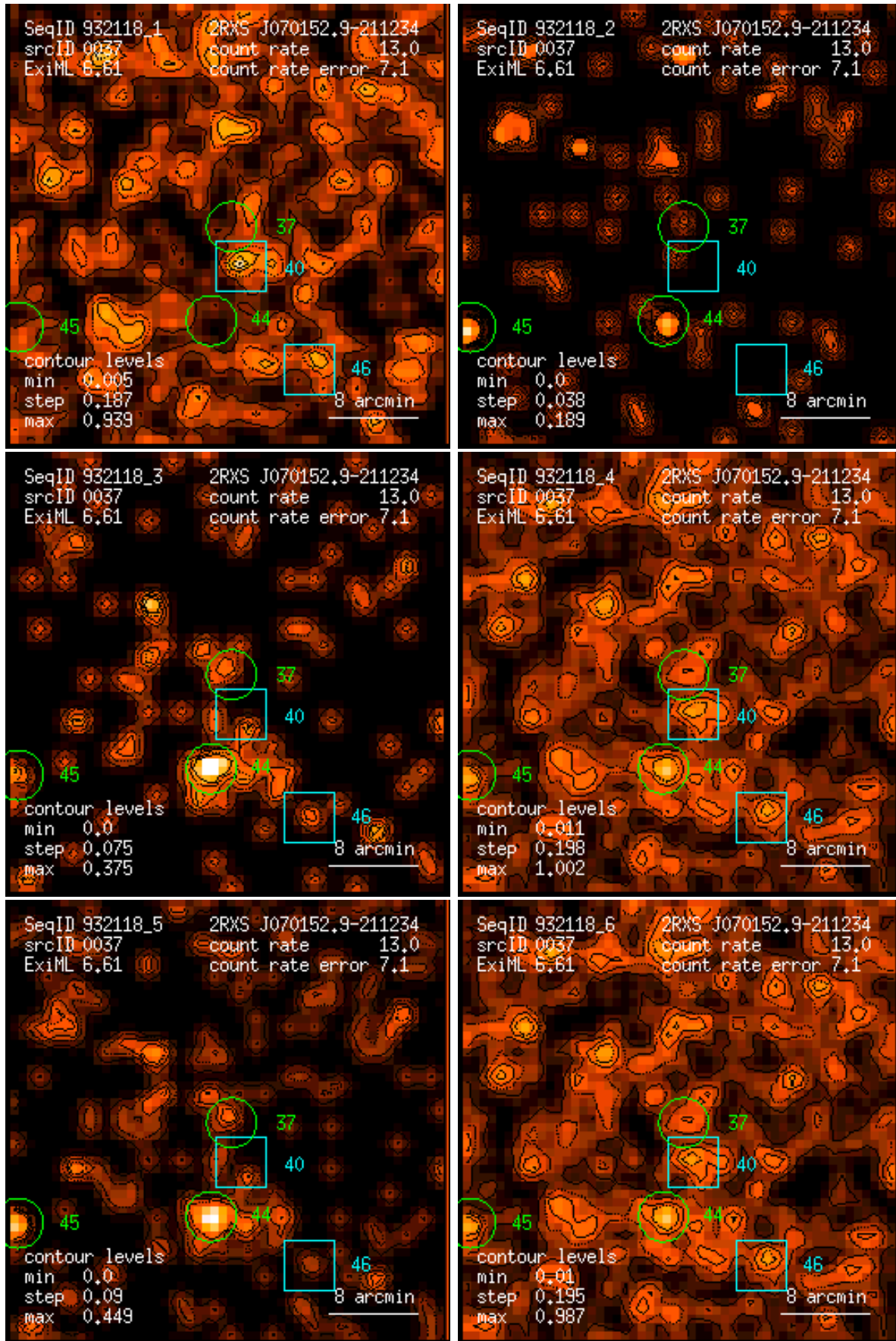
Figure 37: RASS 932118: detection 0037: band rate images, Gaussian filter: (1) PSPC channels 11 – 41, (2) 52 – 90, (3) 91 – 201, (4) 11 – 235, (5) 52 – 201, (6) 11 – 201. Broad band rates in counts/ks. Band rate contour levels in counts/ks/arcmin 2 .
