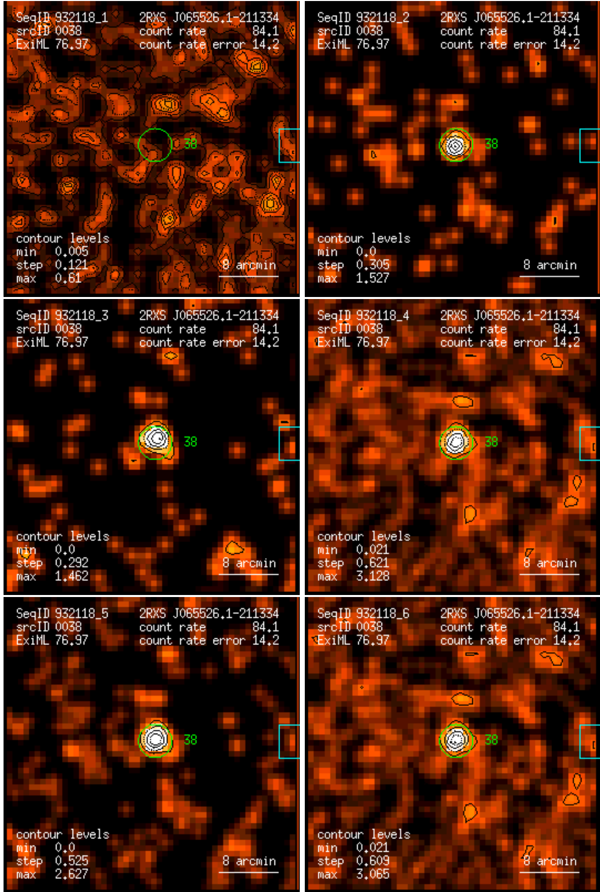
Figure 38: RASS 932118: detection 0038: band rate images, Gaussian filter: (1) PSPC channels 11 – 41, (2) 52 – 90, (3) 91 – 201, (4) 11 – 235, (5) 52 – 201, (6) 11 – 201. Broad band rates in counts/ks. Band rate contour levels in counts/ks/arcmin 2 .
