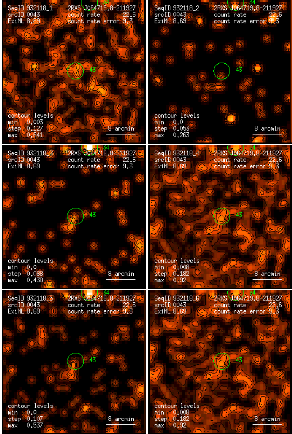
Figure 43: RASS 932118: detection 0043: band rate images, Gaussian filter: (1) PSPC channels 11 – 41, (2) 52 – 90, (3) 91 – 201, (4) 11 – 235, (5) 52 – 201, (6) 11 – 201. Broad band rates in counts/ks. Band rate contour levels in counts/ks/arcmin 2 .
