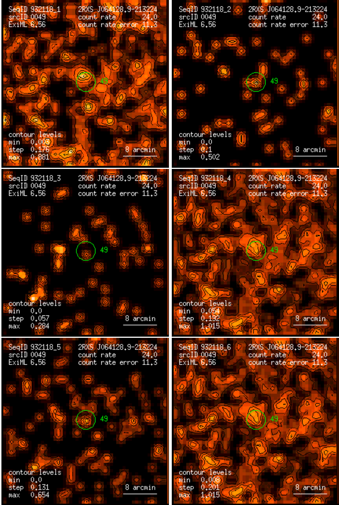
Figure 49: RASS 932118: detection 0049: band rate images, Gaussian filter: (1) PSPC channels 11 – 41, (2) 52 – 90, (3) 91 – 201, (4) 11 – 235, (5) 52 – 201, (6) 11 – 201. Broad band rates in counts/ks. Band rate contour levels in counts/ks/arcmin 2 .
