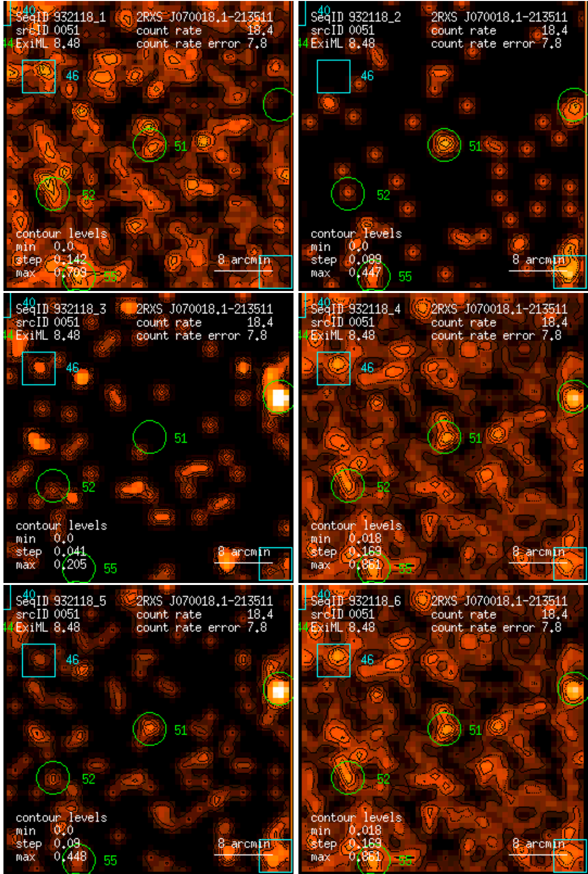
Figure 51: RASS 932118: detection 0051: band rate images, Gaussian filter: (1) PSPC channels 11 – 41, (2) 52 – 90, (3) 91 – 201, (4) 11 – 235, (5) 52 – 201, (6) 11 – 201. Broad band rates in counts/ks. Band rate contour levels in counts/ks/arcmin 2 .
