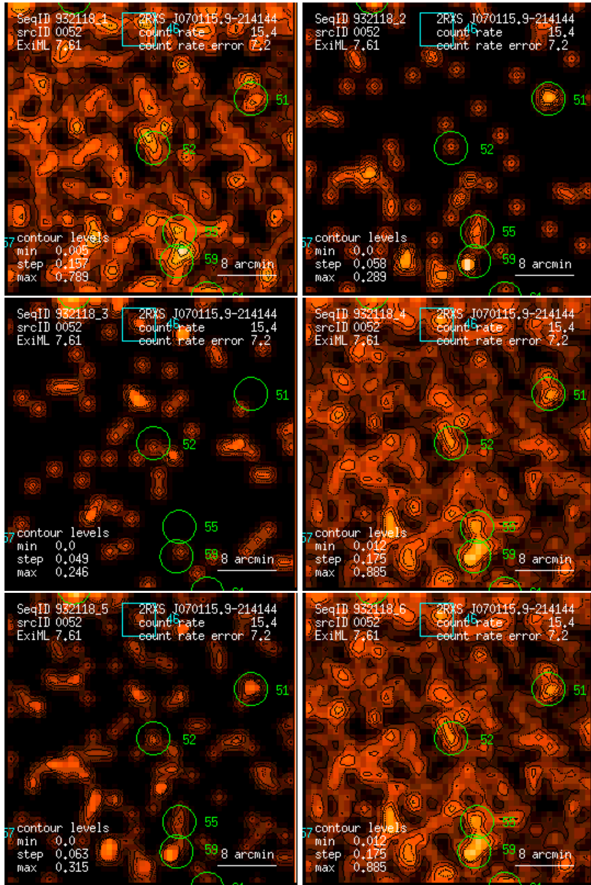
Figure 52: RASS 932118: detection 0052: band rate images, Gaussian filter: (1) PSPC channels 11 – 41, (2) 52 – 90, (3) 91 – 201, (4) 11 – 235, (5) 52 – 201, (6) 11 – 201. Broad band rates in counts/ks. Band rate contour levels in counts/ks/arcmin 2 .
